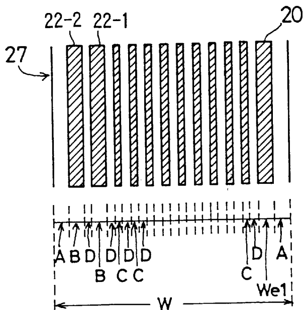
FIG. 13B PRIOR ART
