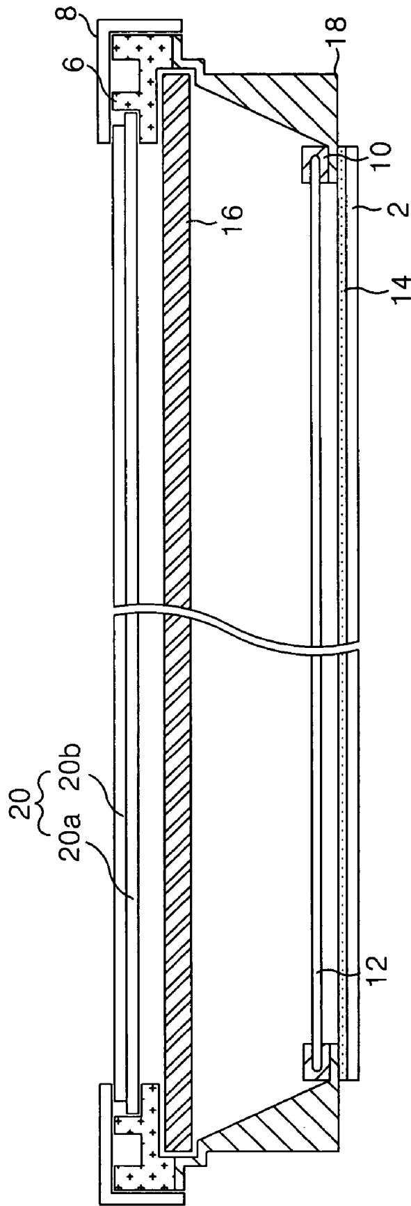
FIG. 1 RELATED ART
