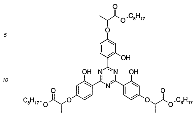
Compound 101
