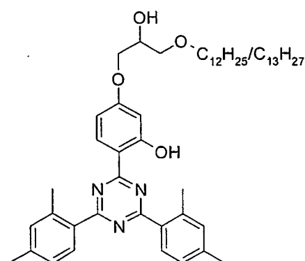
Compound 102
