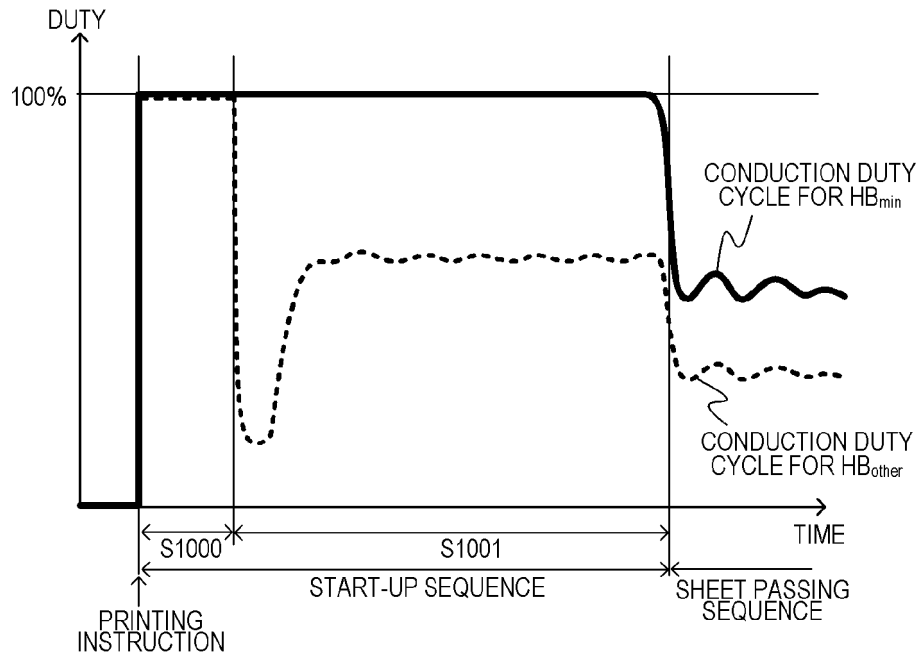
FIG. 6B CONDUCTION DUTY CYCLE
