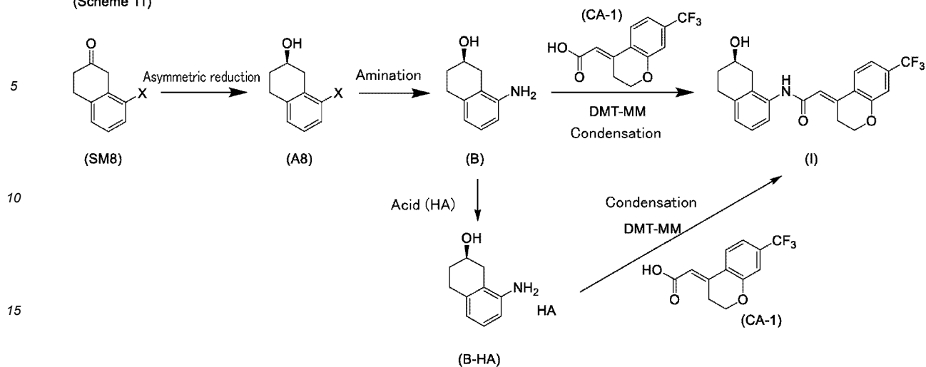
(Scheme 11)
