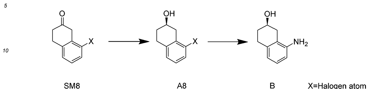
(Scheme C-2)
