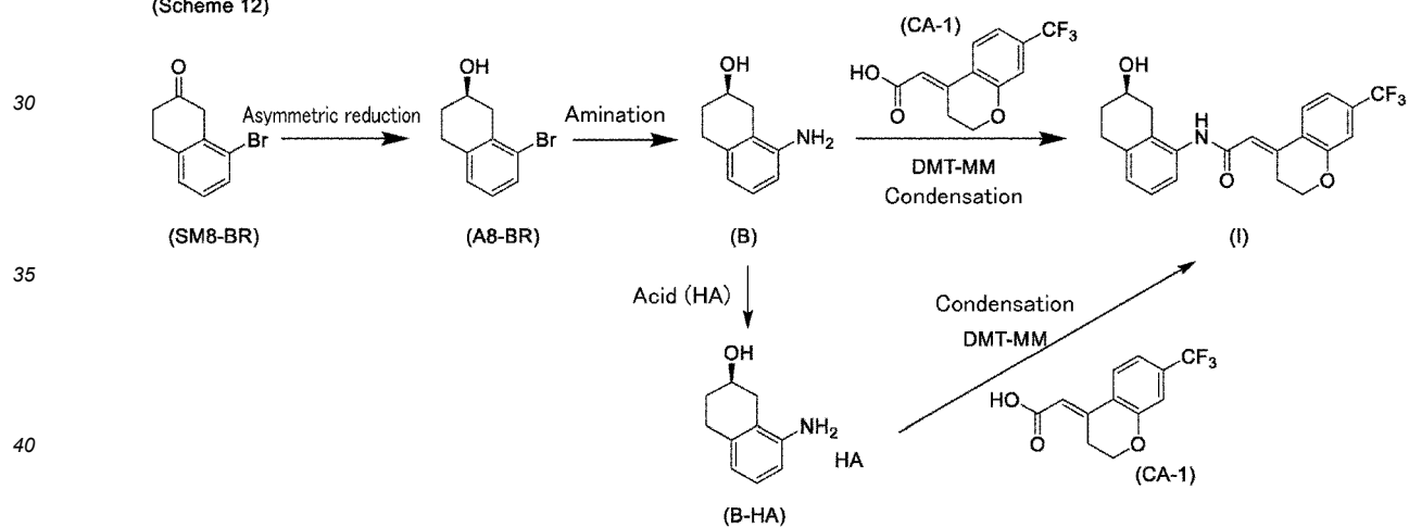
(Scheme 12)
