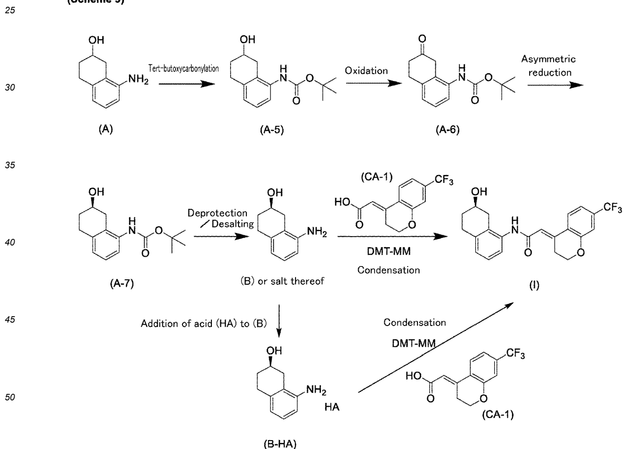
(Scheme 9)
