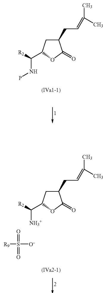
Scheme 5
