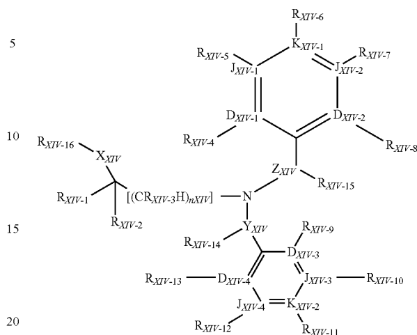
Formula XIV
