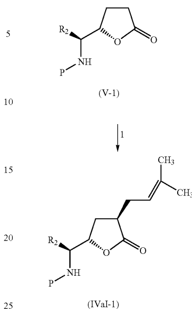
Scheme 3
