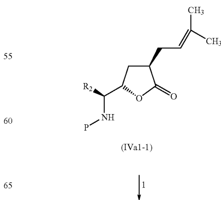
Scheme 4
