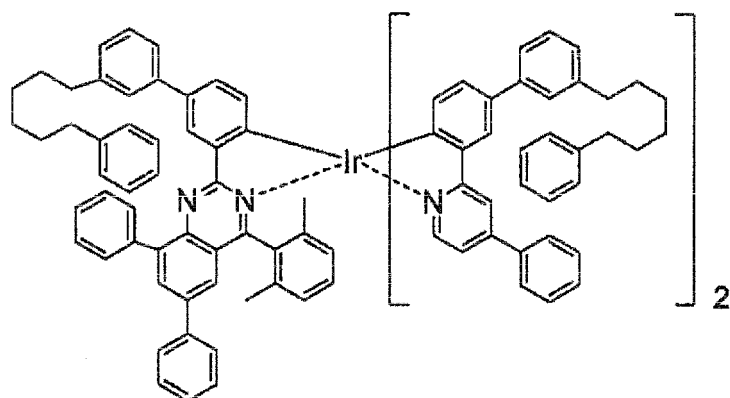
(compound D-4)
