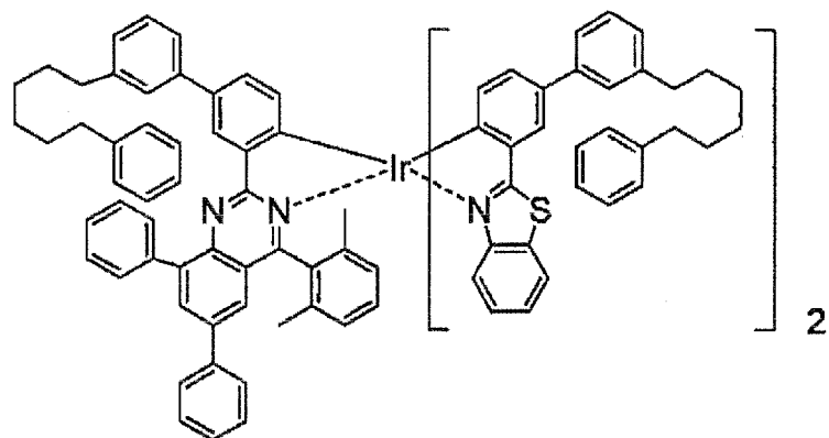
(compound D-3)
