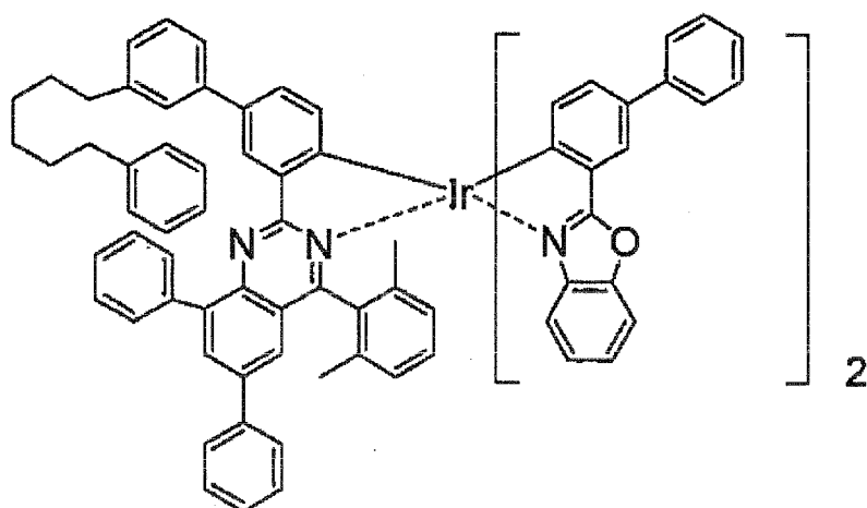
(compound D-2)
