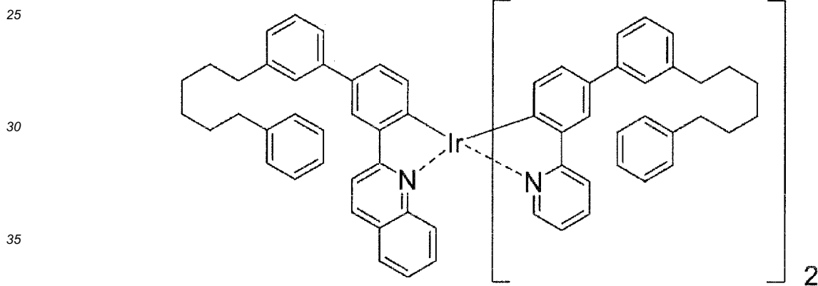
(compound D-8)
