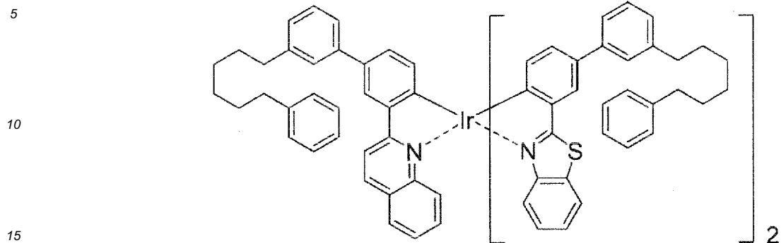
(compound D-7)
