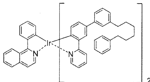
(compound D-10)
