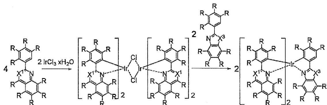
(scheme A)
