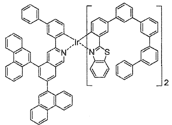
[Chem. 16]
