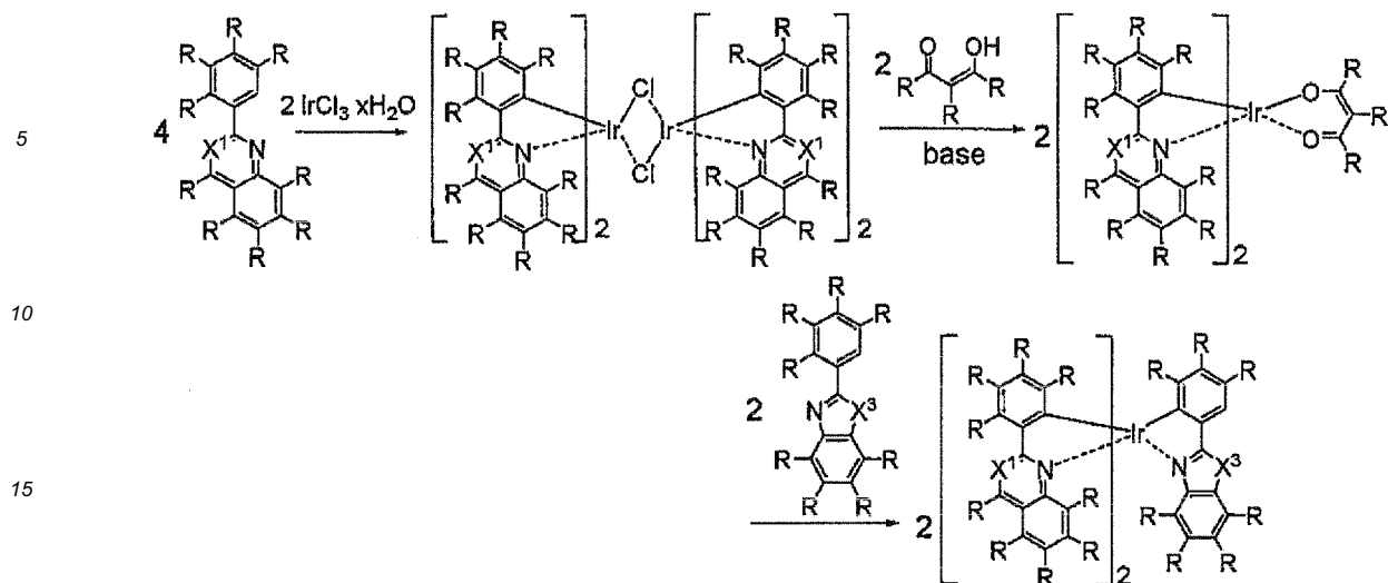
(scheme B)
