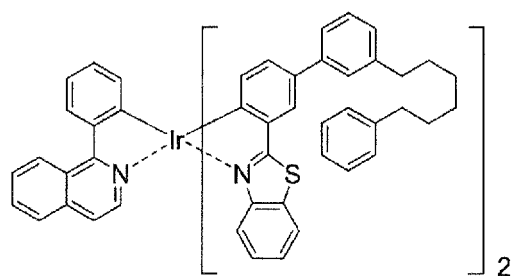
(compound D-9)
