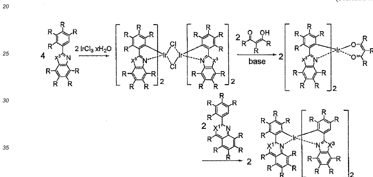
(scheme C)
