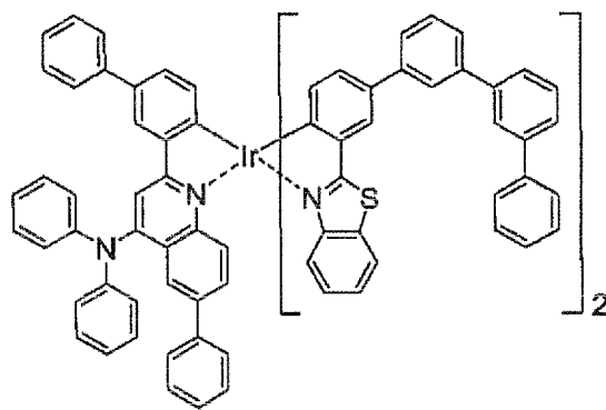
[Chem. 14]
