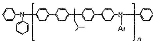
(PB-2)
