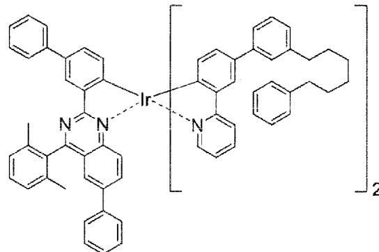
(compound D-6)
