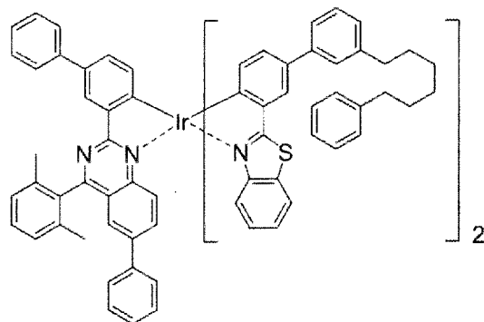
(compound D-5)
