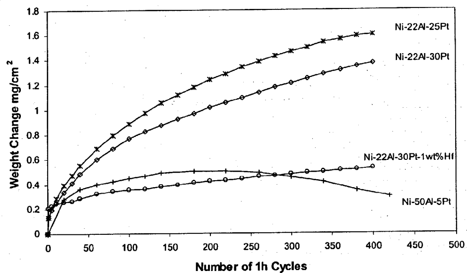
Figure 11 Comparison of the cyclic oxidation kinetics of Pt-modified \beta -NiAl, Pt-modified \gamma' -Ni 3 Al + \gamma -Ni, and Pt modified \gamma' -Ni 3 Al + \gamma -N with Hf at 1150°C in air.
