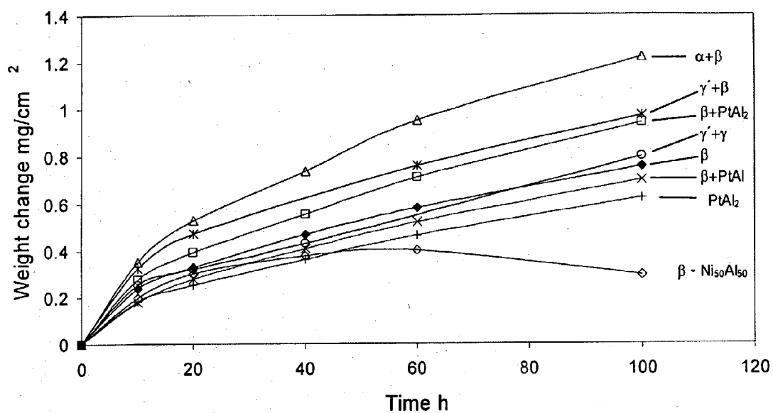
Figure 6 Weight change of Ni-Al-Pt alloys of different phase constitutions after "isothermal" exposure at 1150°C in still air. Also included for comparison is binary β-NiAl of stoichiometric composition.
