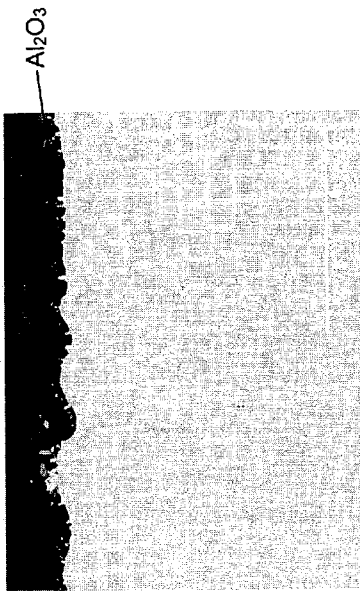
#7: Ni-22Al-30Pt (500h)
