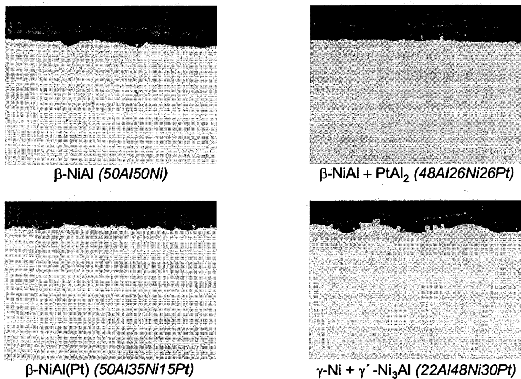
Figure 7 Cross-sectional images of selected alloys shown in Fig. 6 after 100 h oxidation at 1150°C in air. The compositions are nominal and in atom percent.
