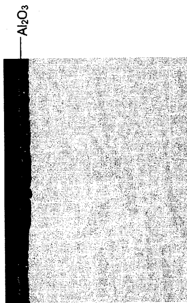
#27: Ni-22Al-20Pt (500h)
