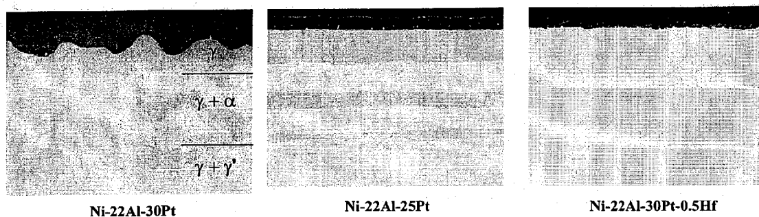
Figure 8 Cross-sectional images of selected \gamma' + \gamma alloys after 1000 h isothermal oxidation at 1150°C in air. All images are the same magnification (x500). The compositions are nominal and in atom percent.
