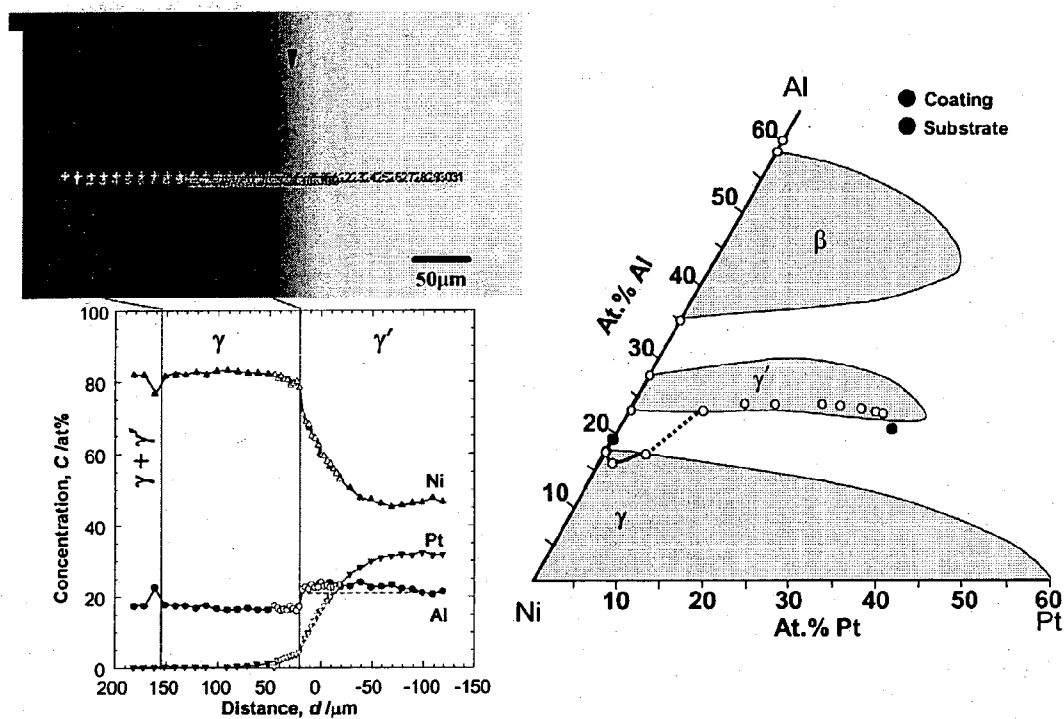
Figure 18 Microstructure and composition profiles through a \gamma'+\gamma (Ni-22Al-30Pt)/ \gamma'+\gamma (Ni-22Al) couple after 50 h interdiffusion at 1150°C.
