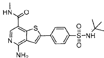
6TP 4-amino-2-[4-(tert-butylsulfamoyl)phenyl]-N-methylthieno[3,2-c]pyridine-7-carboxamide Thienopyridine 19
