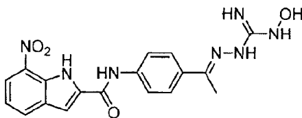
XK9 N-[4-[(1E)-N-(N-hydroxycarbamimidoyl)ethanehydrazono]phenyl]-7-nitro-1H-indole-2-carboxamide;
