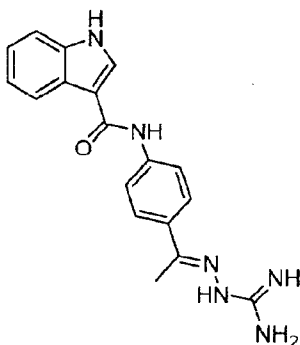
NXP N-[4-[(1E)-N-CARBAMIMIDOYLETHANEHYDRAZONOYL]PHENYL]-1H-INDOLE-3-CARBOXAMIDE
