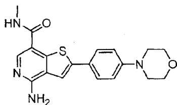
0TP 4-amino-N-methyl-2-[4-(morpholin-4-yl)phenyl]thieno[3,2-c]pyridine-7-carboxamide Thienopyridine 8
