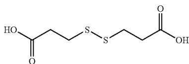
3,3'-disulfanediyldipropanoic acid
