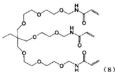
[Chemical Formula 8]
