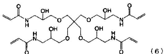
[Chemical Formula 6]
