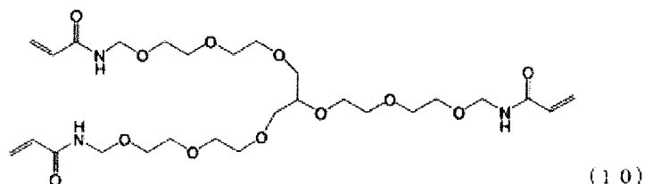
[Chemical Formula 10]
