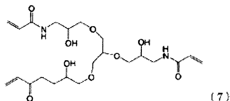
[Chemical Formula 7]
