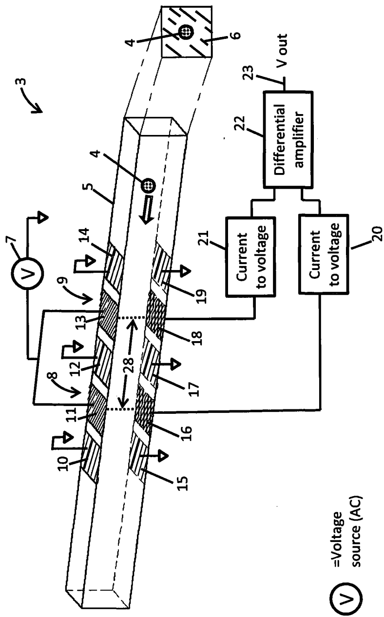
Figure 5. Block diagram to perform measurement for new electrode design.
