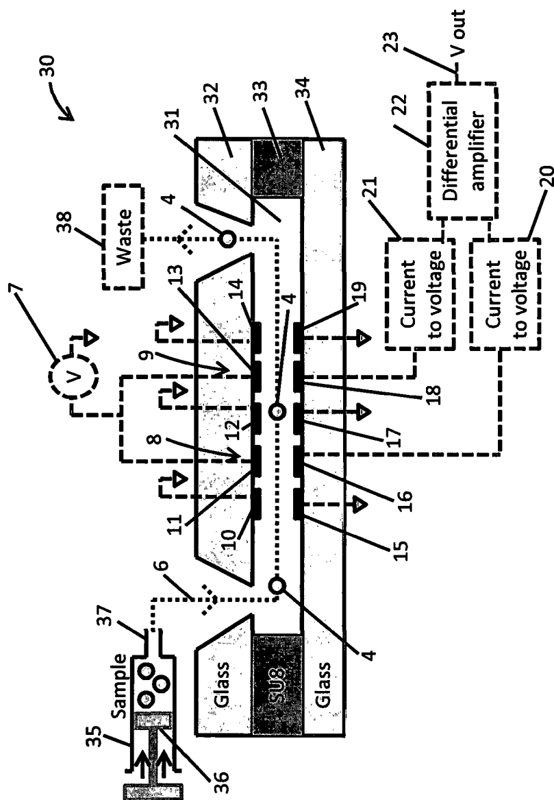
Figure 8. Overview of operation of the new electrode design.
