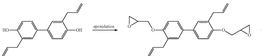
[Reaction 1]
