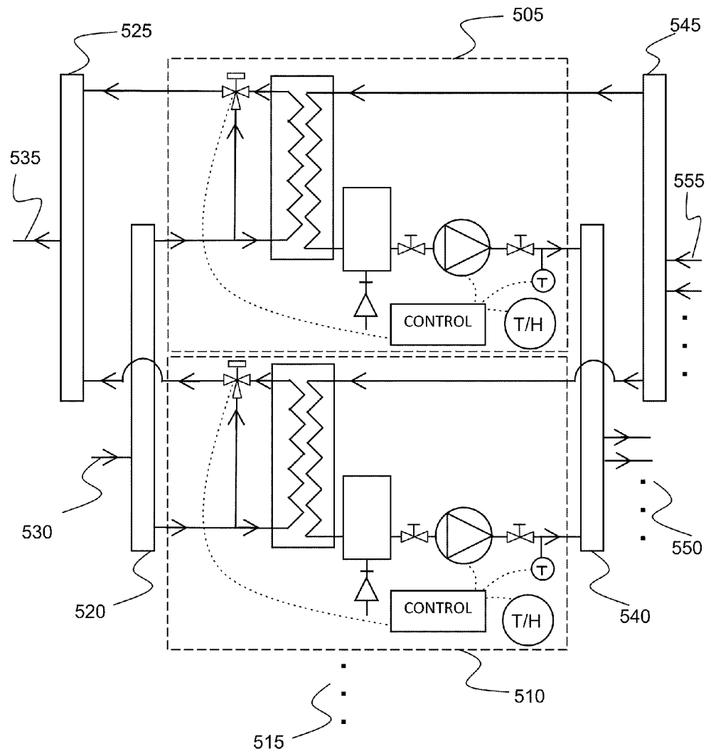
MODULAR CDU INTERCONNECTION MULTIPLE RACKS FIG. 5
