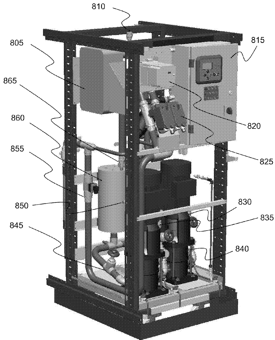
FRONT PERSPECTIVE VIEW FLOOR-MOUNT CDU FIG. 8
