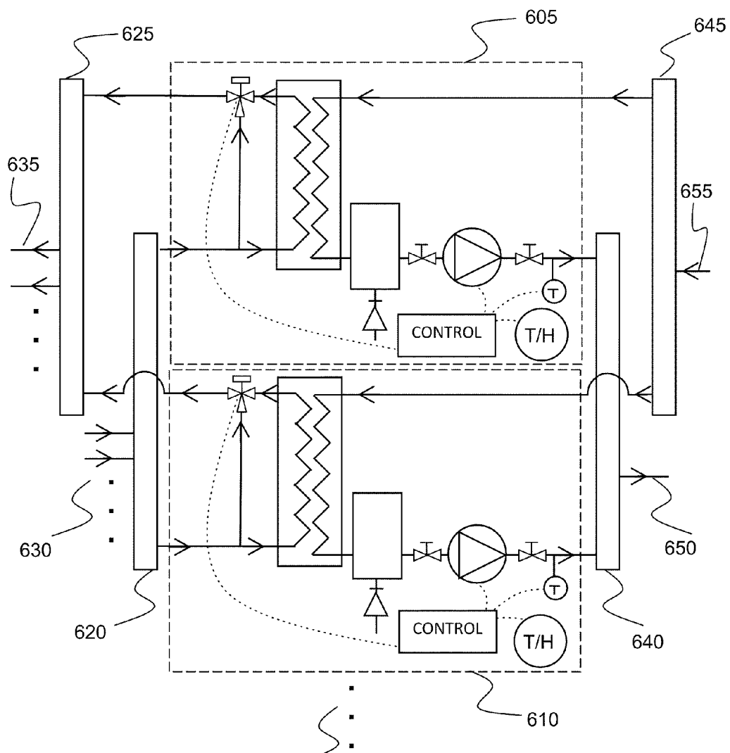
615 MODULAR CDU INTERCONNECTION MULTIPLE SOURCES FIG. 6
