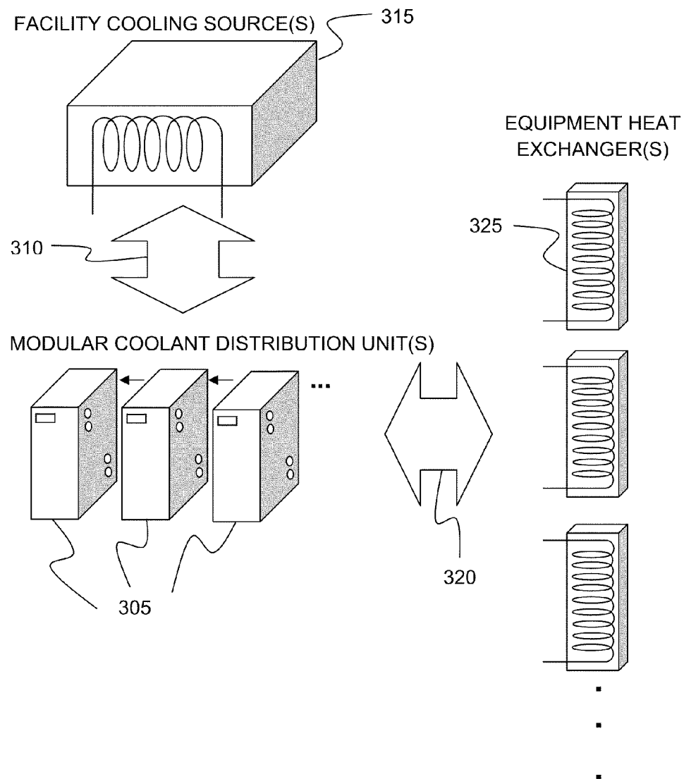
Modular Free Cooling System Overview FIG. 3
