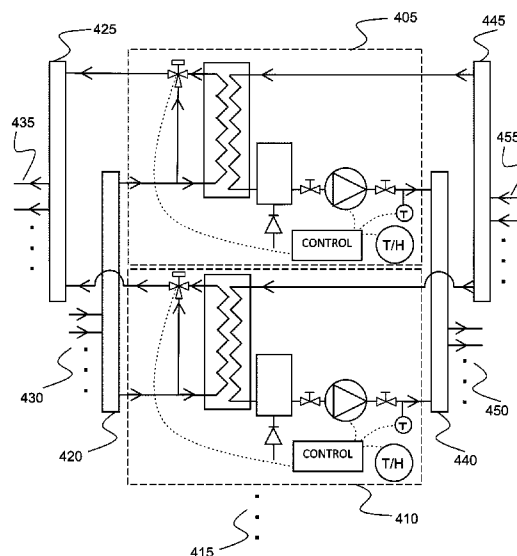
MODULAR CDU INTERCONNECTION MULTIPLE SOURCES, MULTIPLE RACKS, WITH MANIFOLDS
