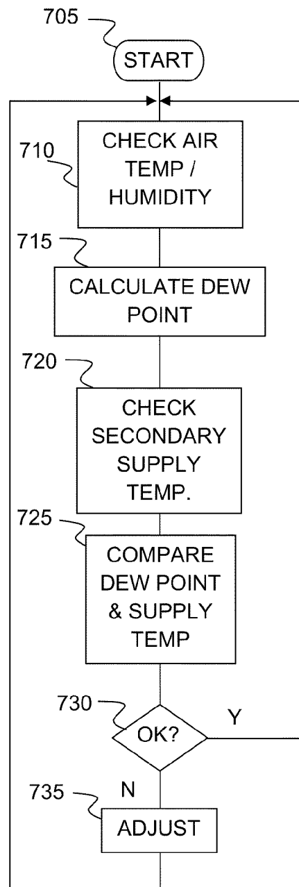
MODULAR SCALABLE OPERATION FLOW CHART FIG. 7
