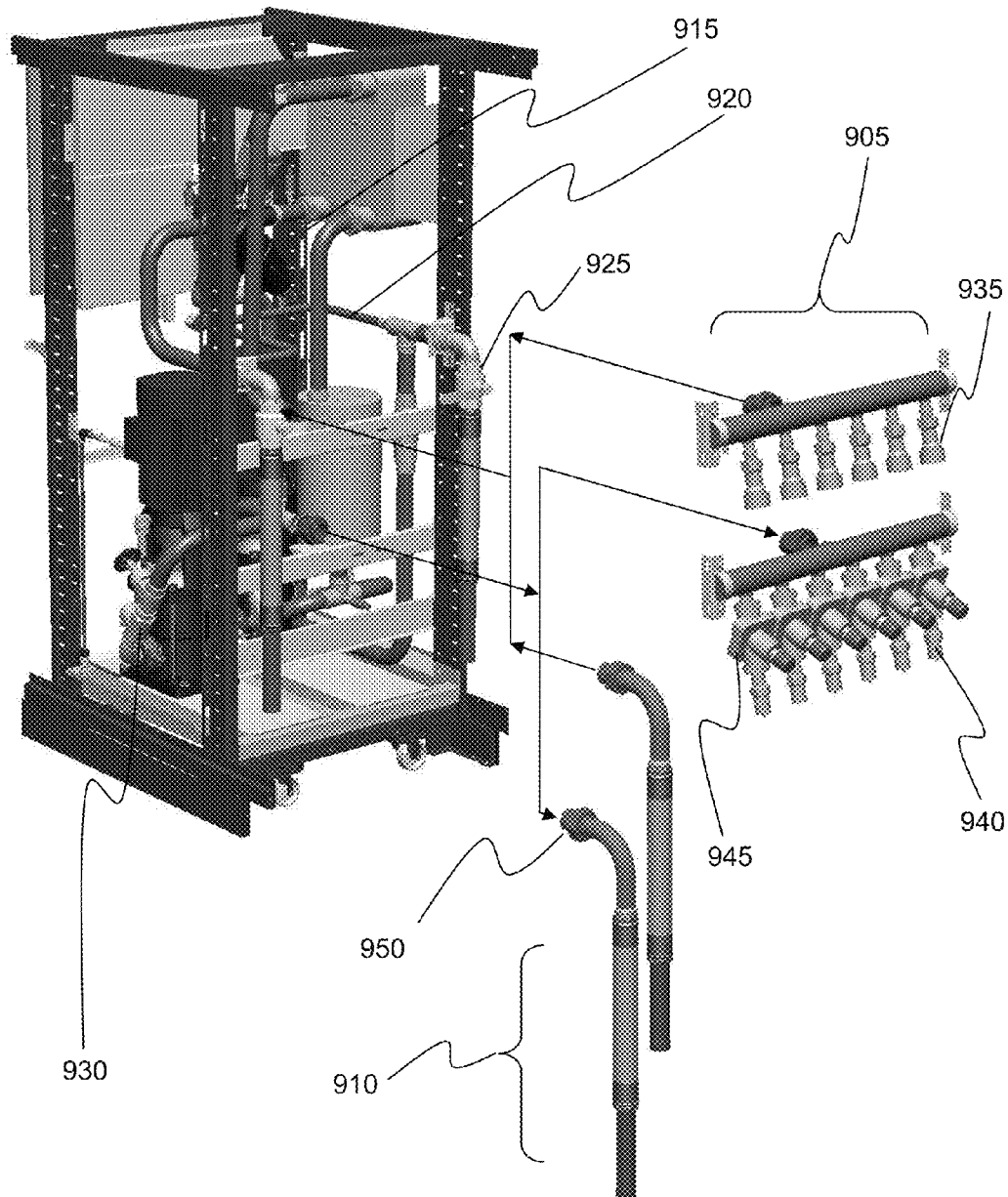
REAR PERSPECTIVE VIEW FLOOR-MOUNT CDU FIG. 9
