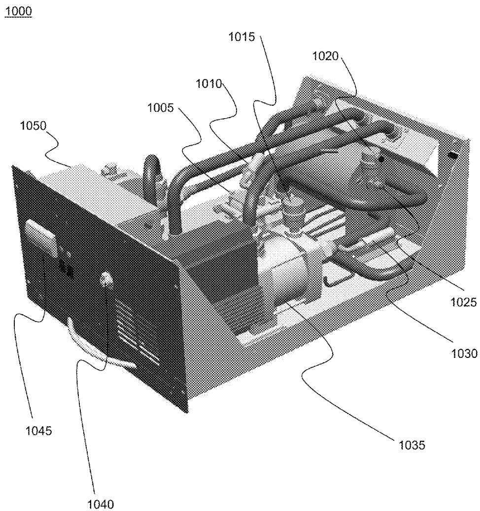
FIRST PERSPECTIVE VIEW RACK-MOUNT CDU FIG. 10
