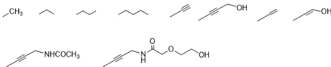
STRUCTURES XIX-XXVIII
