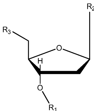
Structure I
