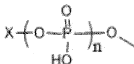
Structure XIV
