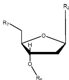
Structure IV
