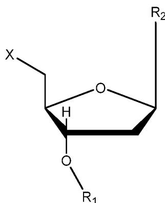
Structure III
