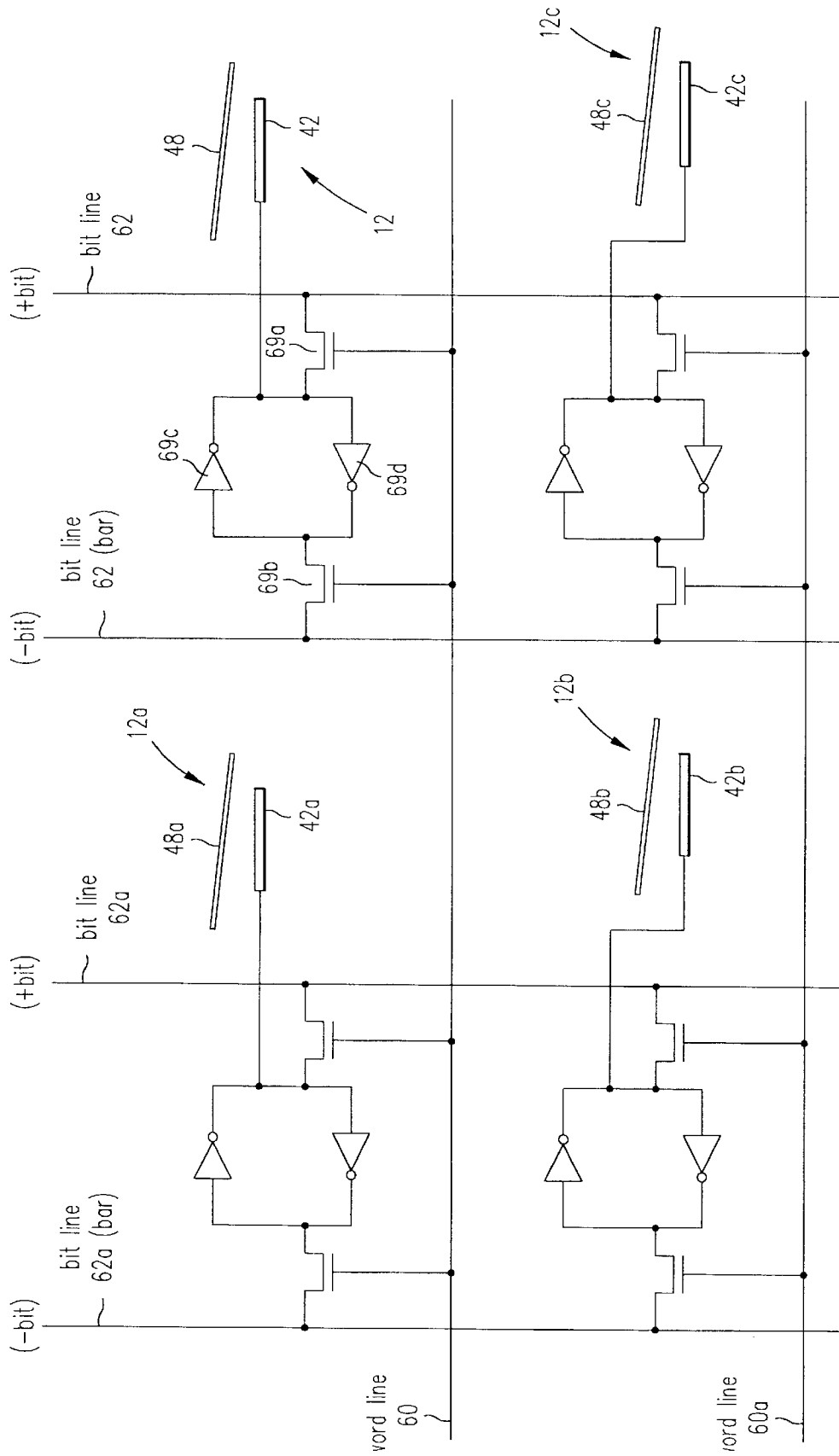
SRAM Implementation
