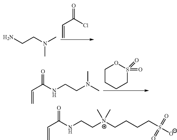
C4 Sulfobetaine ZALs, differing the spacing between the zwitterionic charge
