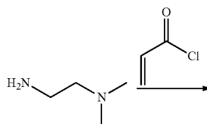
C4 Sulfobetaine ZALs, differing the spacing between the zwitterionic charge
