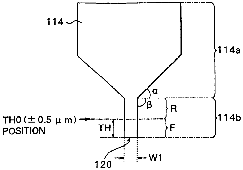
FIG. 45 PRIOR ART
