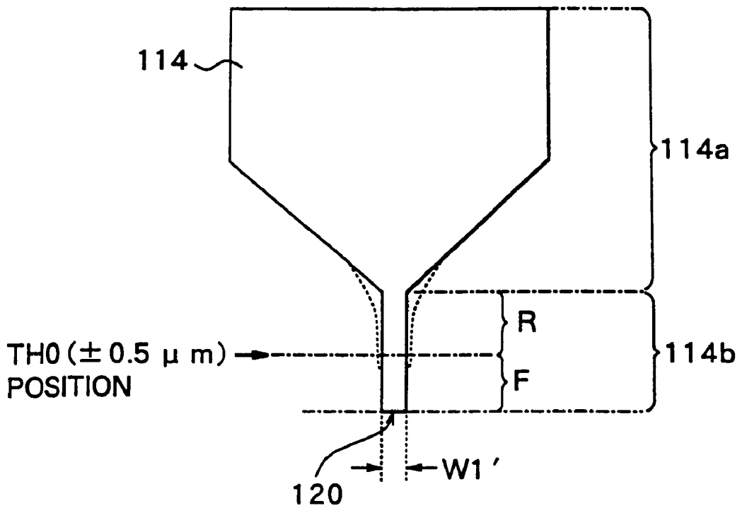
FIG. 46 PRIOR ART
