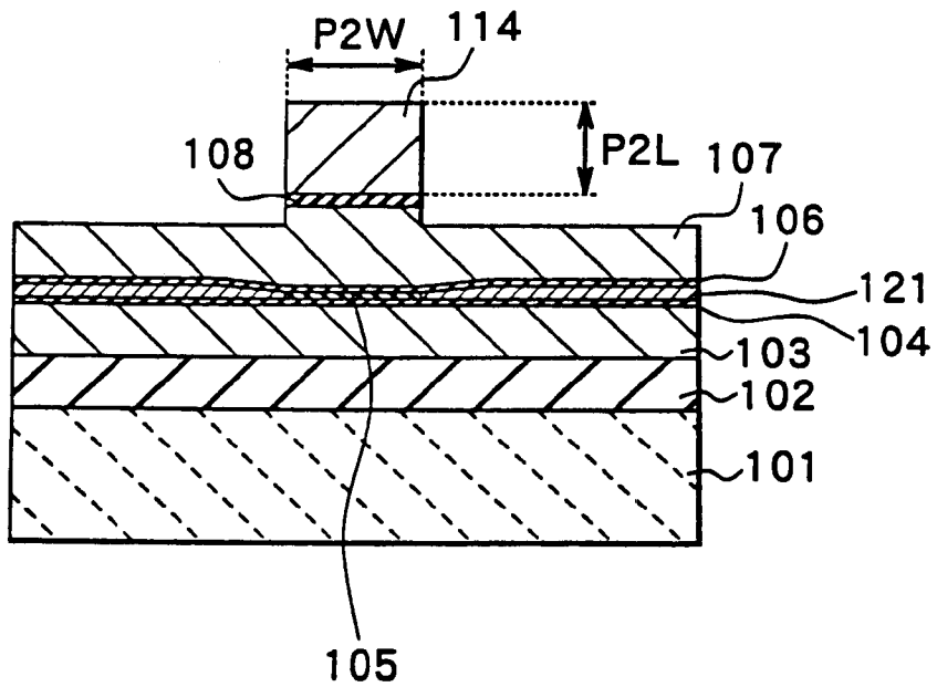
FIG.43 PRIOR ART
