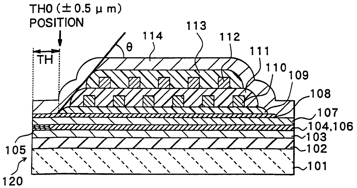
FIG.42 PRIOR ART
