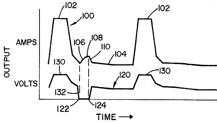
FIG. 2 (PRIOR ART)
