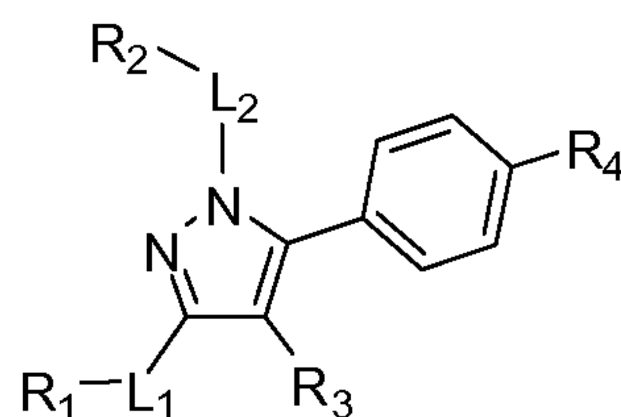
Formula (V);
