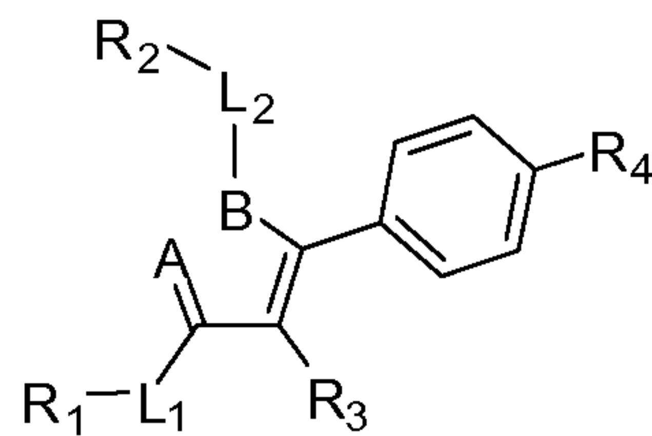
Formula (E);
