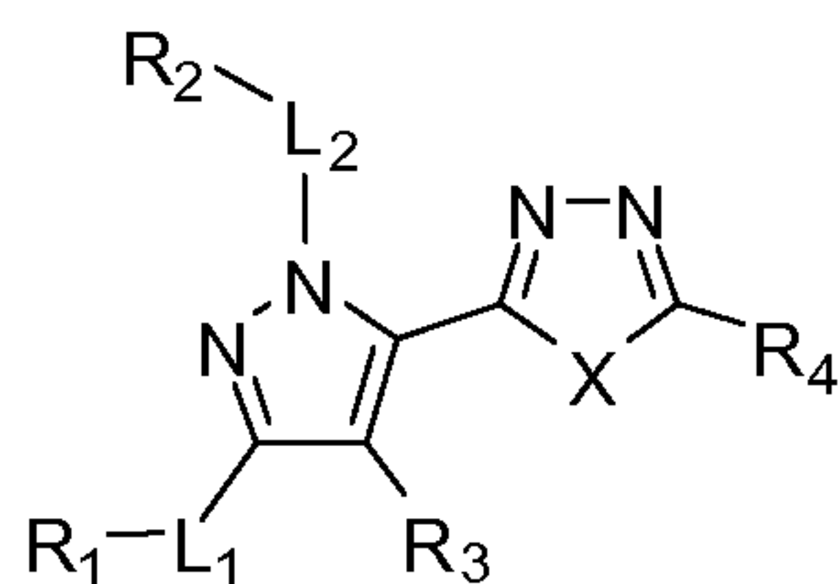
Formula (I);
