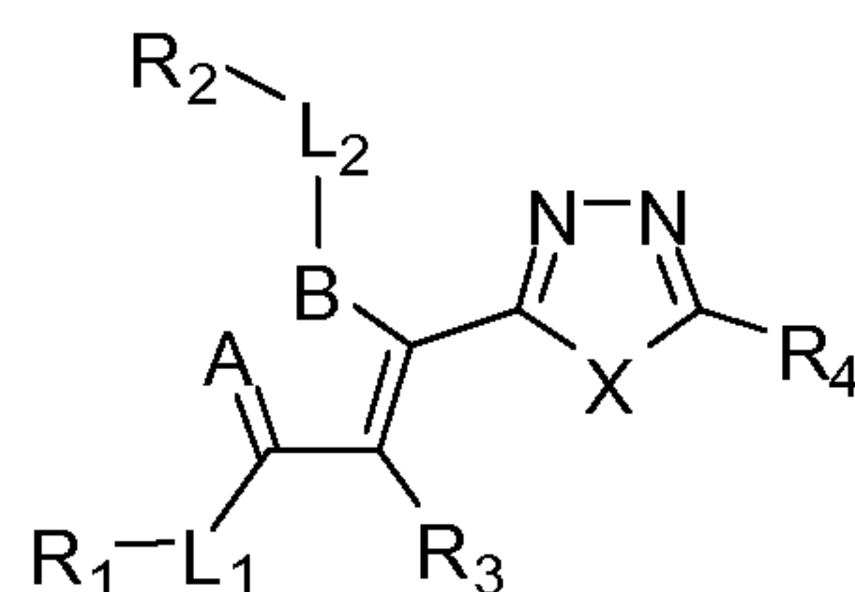
Formula (A);
