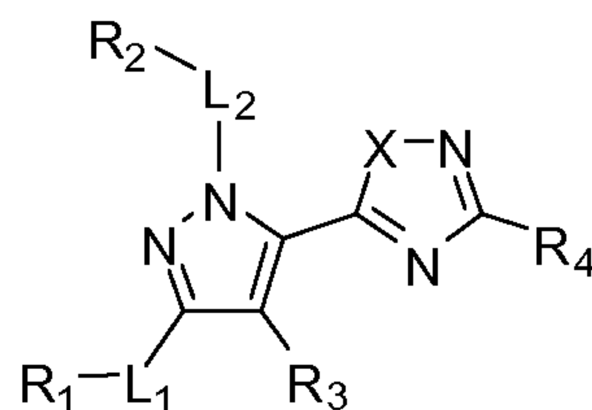
Formula (II);
