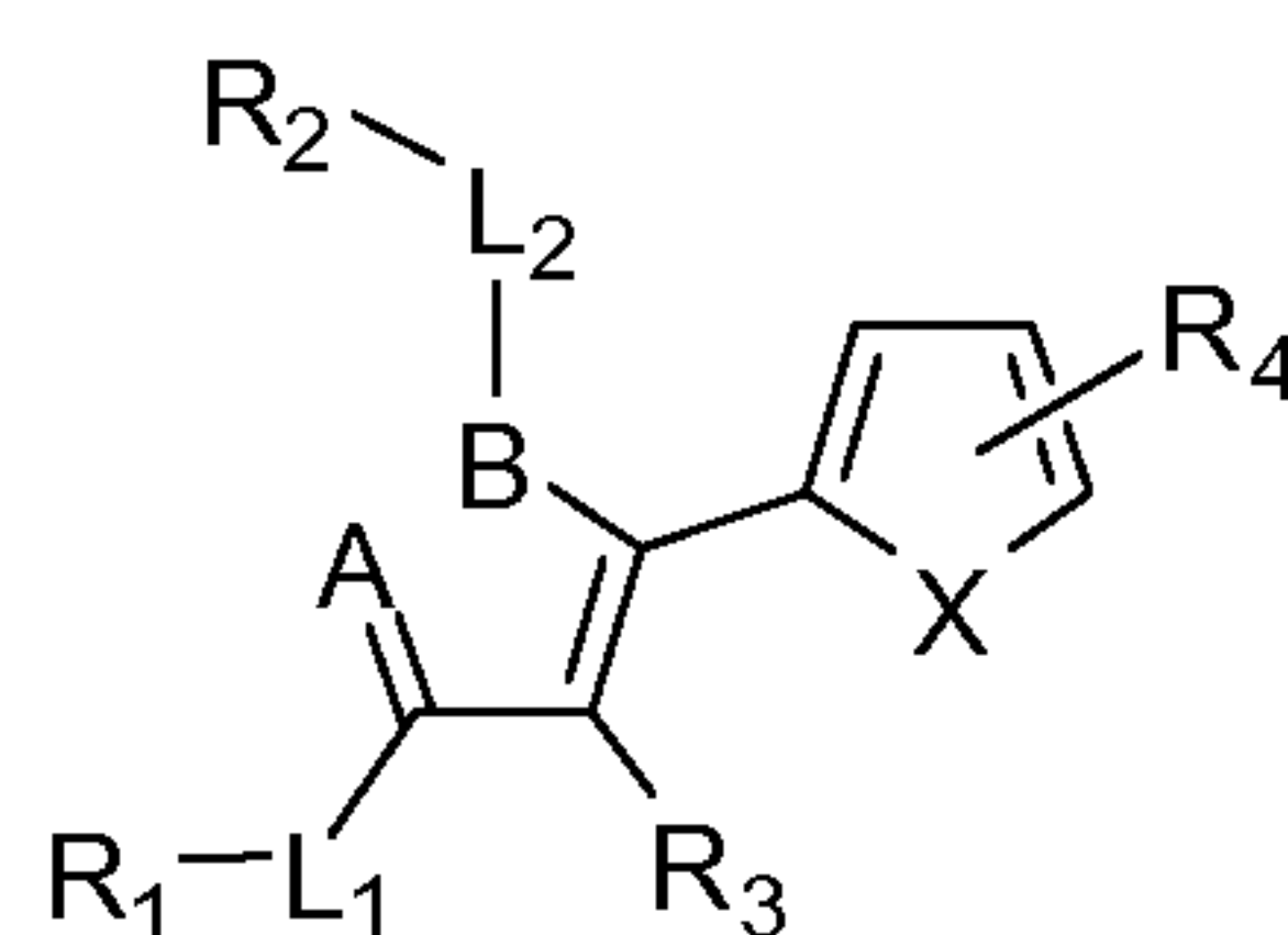
Formula (F);
