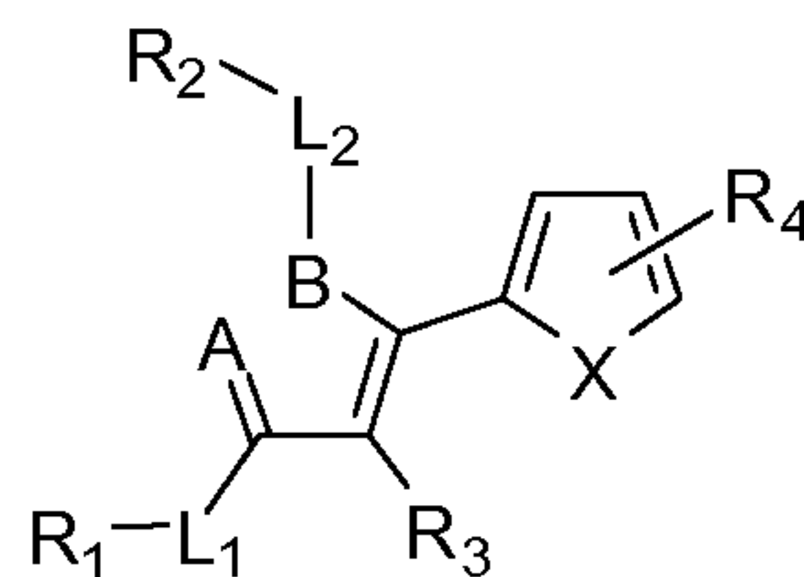
Formula (F);
