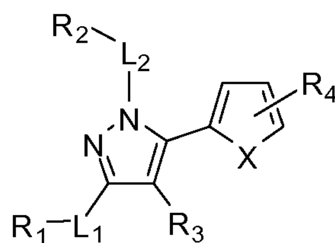
Formula (IV);
