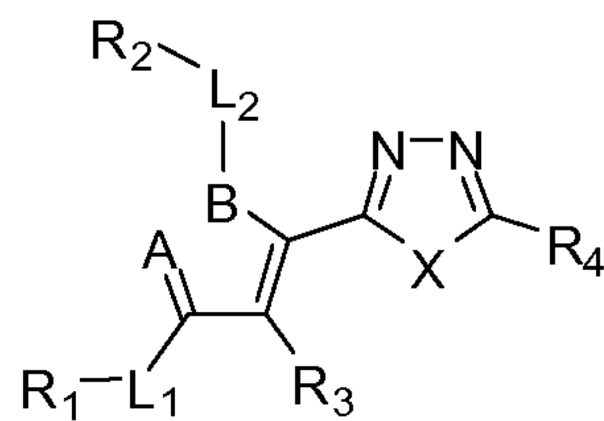
Formula (A);
