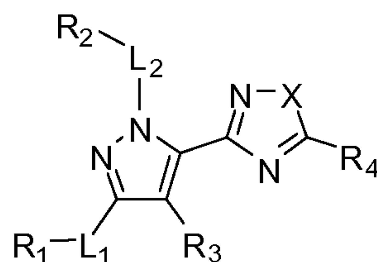
Formula (III);
