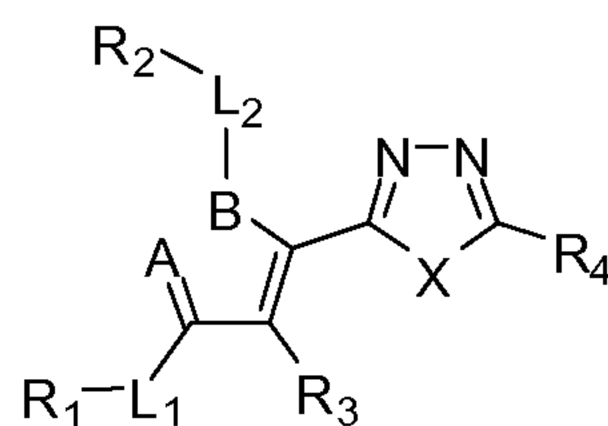
Formula (A);
