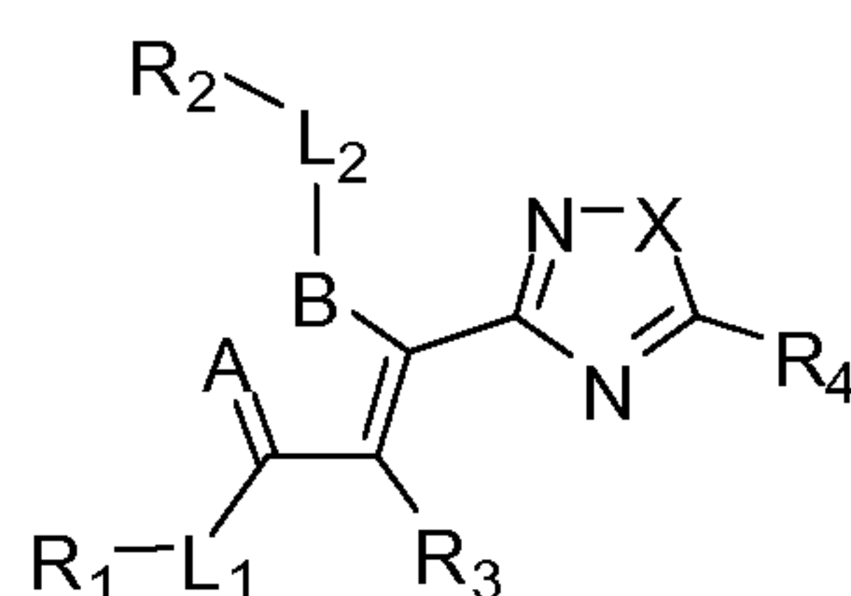
Formula (C);
