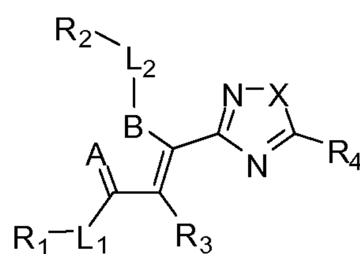
Formula (C);
