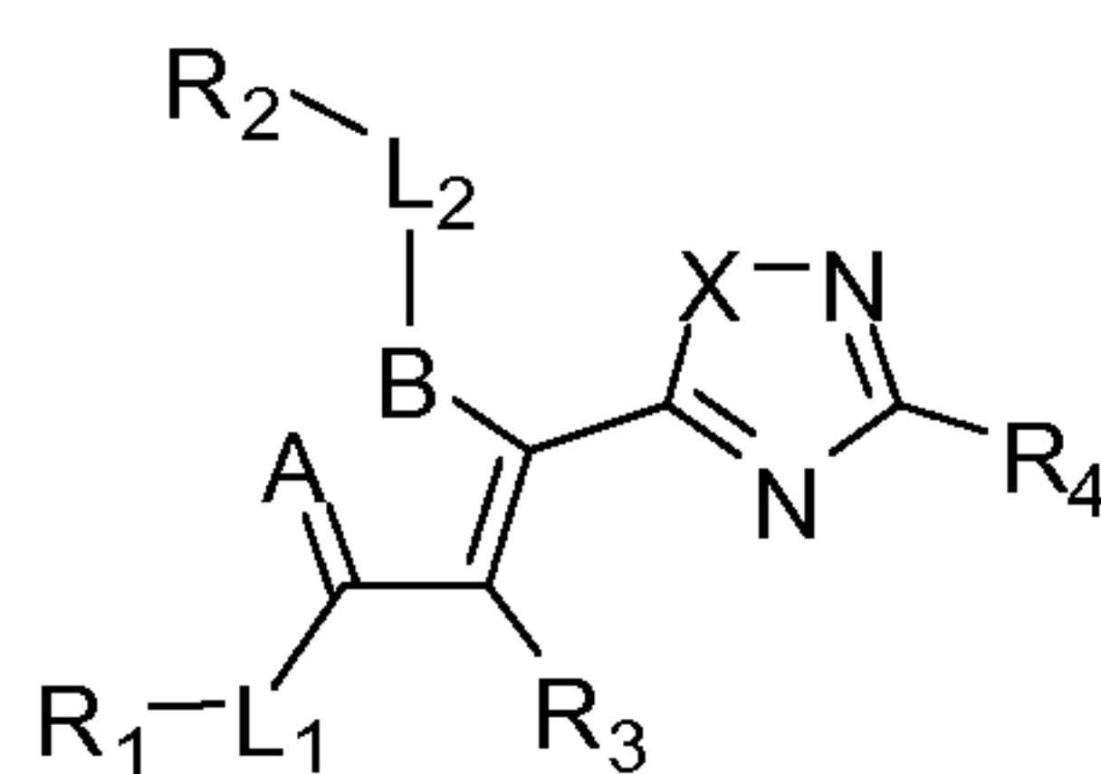
Formula (B);
