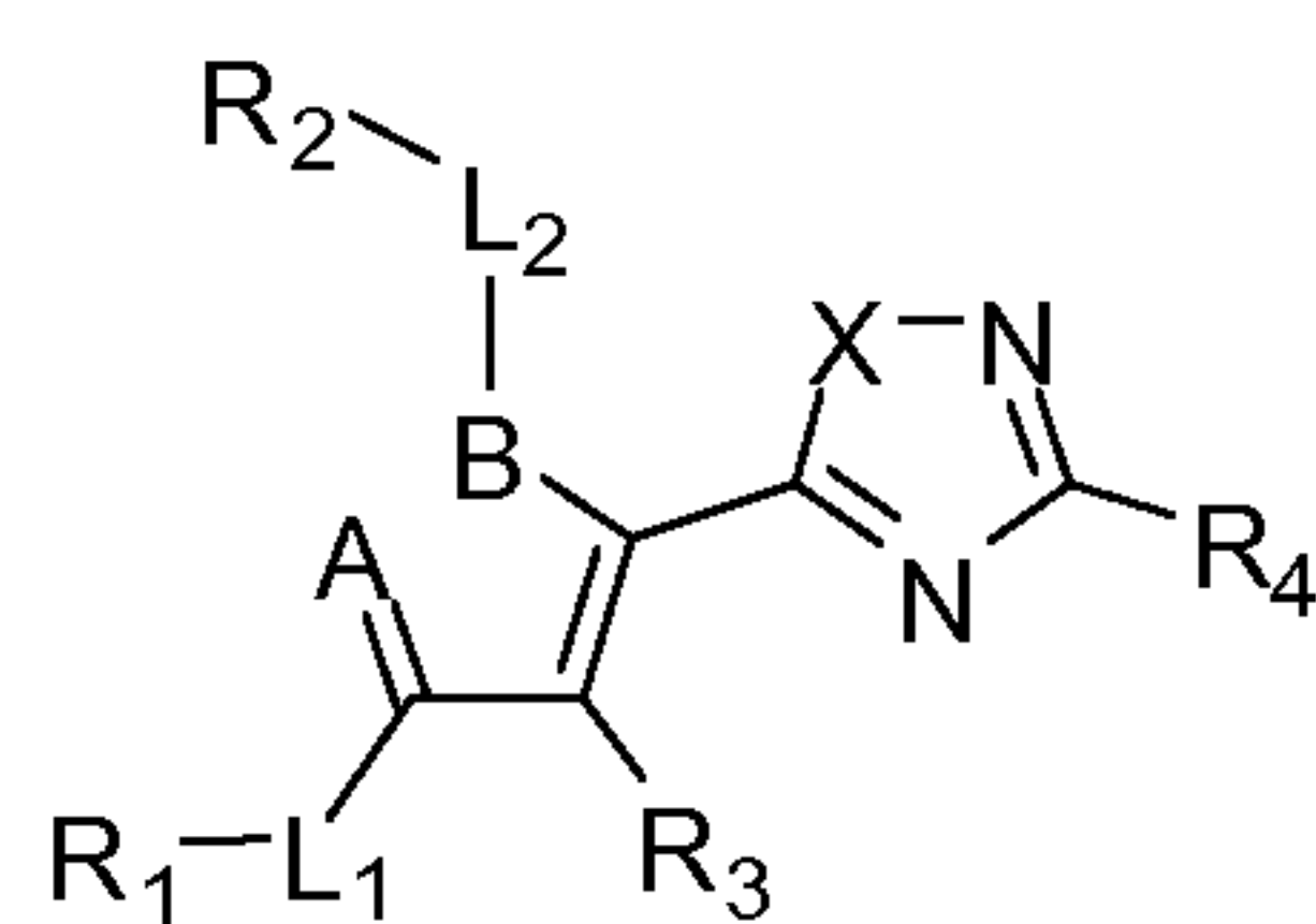
Formula (B);
