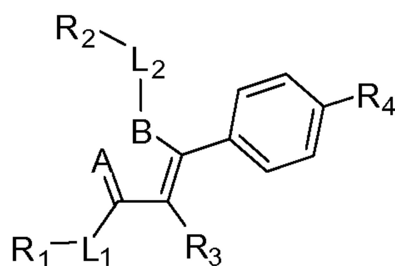
Formula (E);
