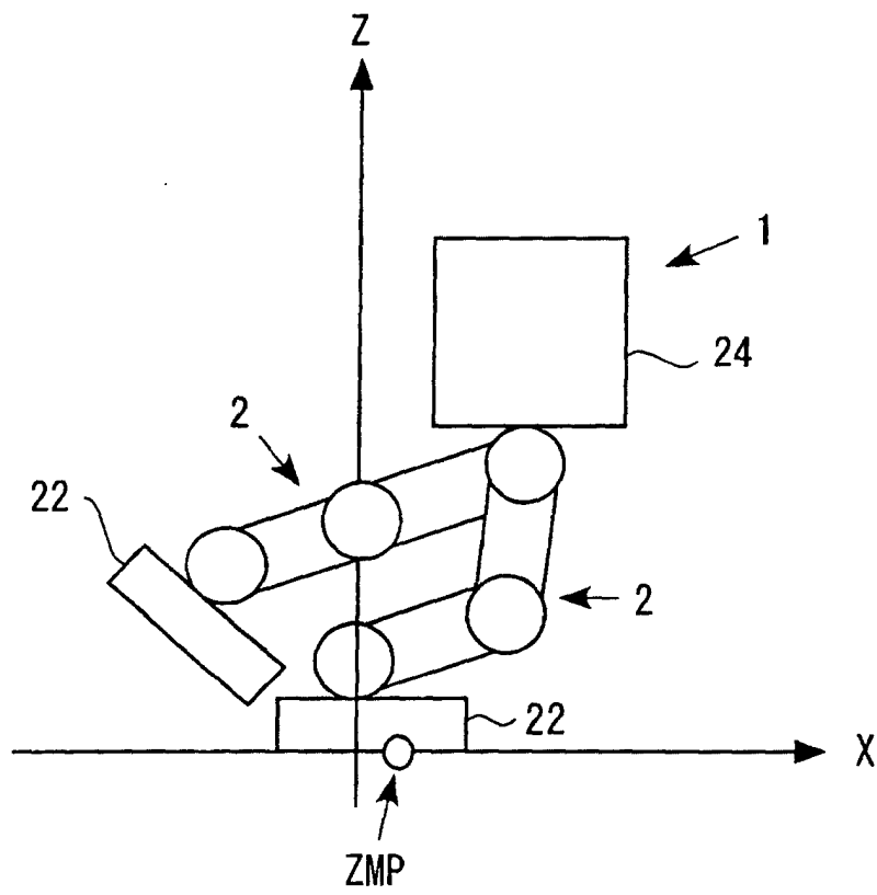
FIG.13 ( DIVERGENCE STATE OF BODY POSITION )
