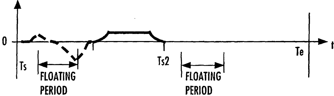
FIG.27 BODY INCLINATION ANGULAR ACCELERATION \beta (FOR RETURNING BODY INCLINATION VELOCITY TO INITIAL VALUE)
