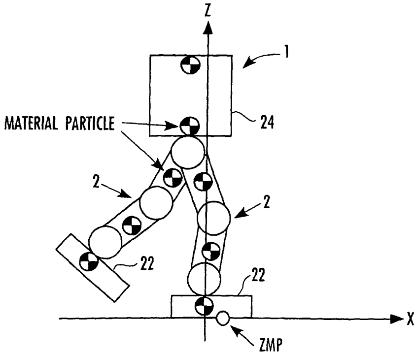
FIG.11 ( FULL MODEL )
