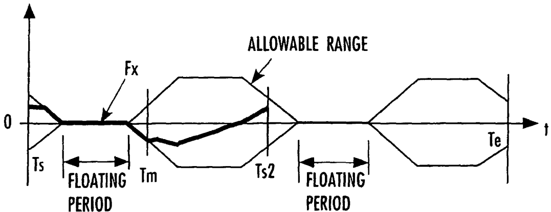
FIG.28 FLOOR REACTION FORCE HORIZONTAL COMPONENT F_x DETERMINED TAKING FLOOR REACTION FORCE HORIZONTAL COMPONENT ALLOWABLE RANGE INTO CONSIDERATION
