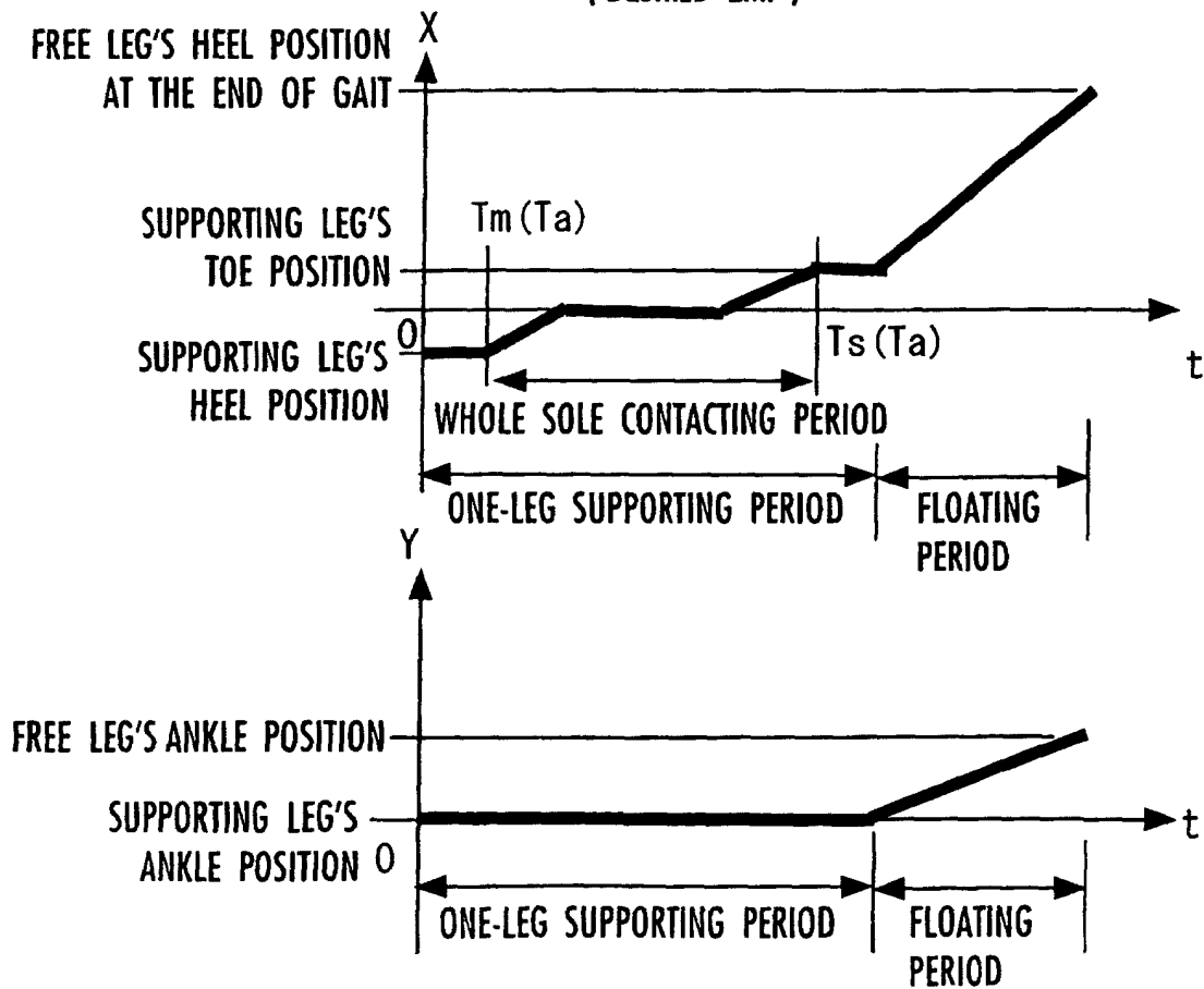
FIG.7 ( DESIRED ZMP )
