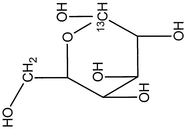
[1- 13 C]-glucose
