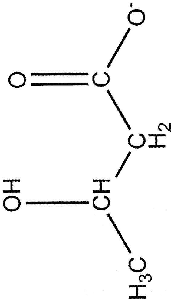
[2,4- 13 C]-β-hydroxybutyrate
