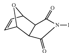
exo-7-oxanorbornene-5,6-dicarboxylic imide (C1)
