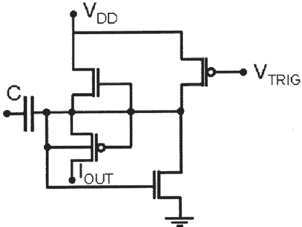
Compact CMOS Programmable Trigger Circuit
