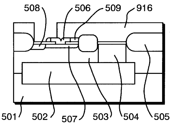
FIG. 9C (PRIOR ART)
