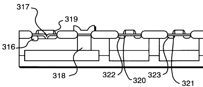
FIG. 6C (PRIOR ART)
