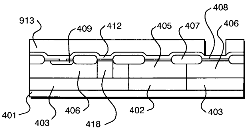
FIG. 7C (PRIOR ART)
