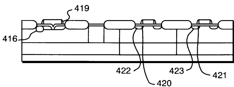
FIG. 8C (PRIOR ART)
