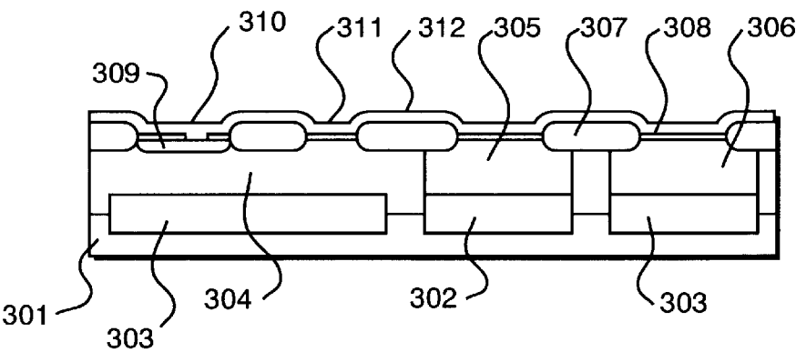
FIG. 5C (PRIOR ART)
