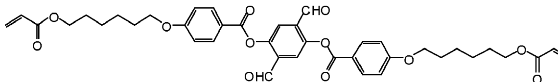
Intermediate C
