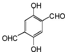
Intermediate B
