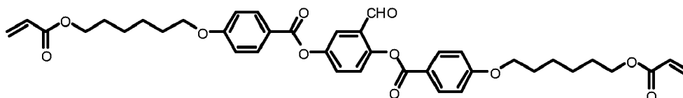
Intermediate D
