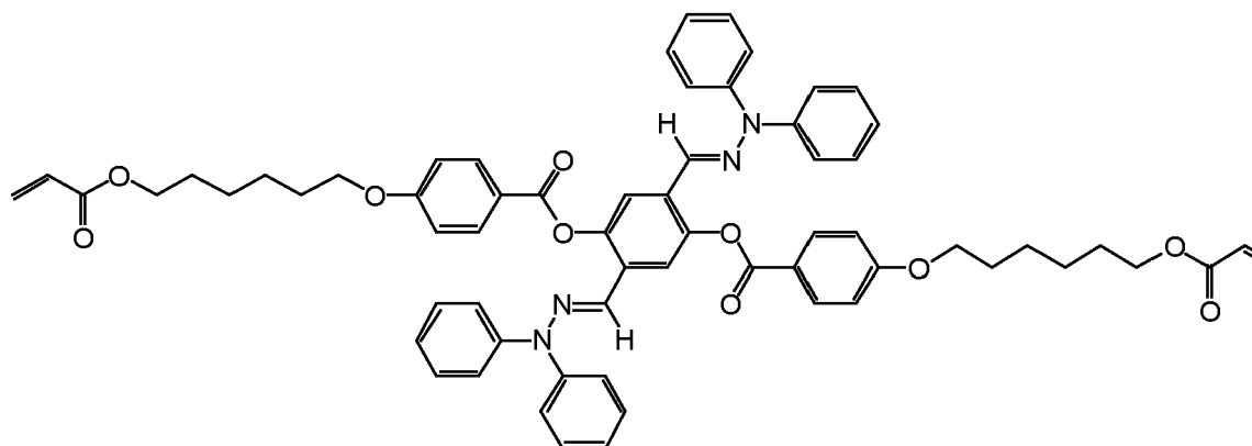
Compound 3
