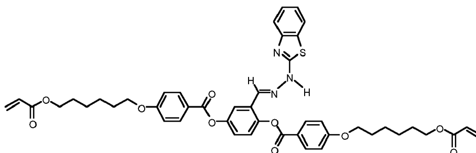
Compound A
