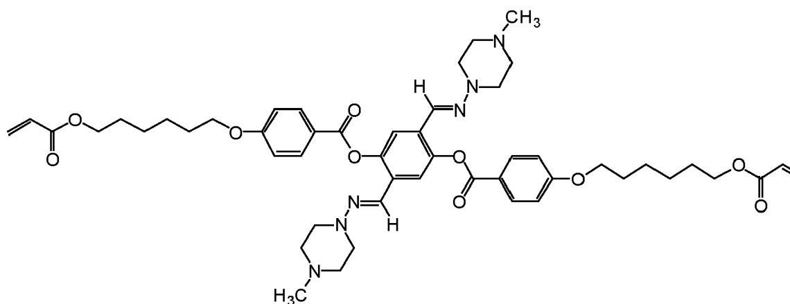
Compound 2
