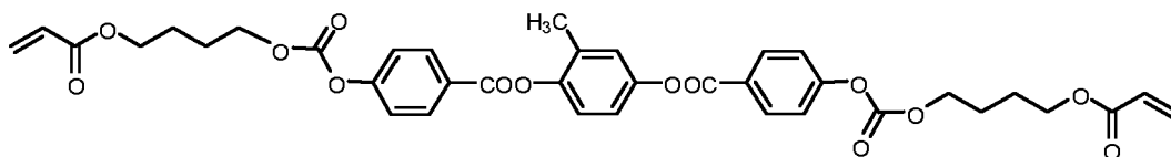
Compound 2r
