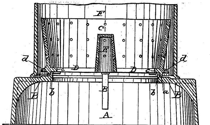
Fig. 2. Section on A-B.
