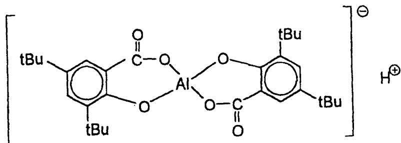
Aluminum complex (9):
