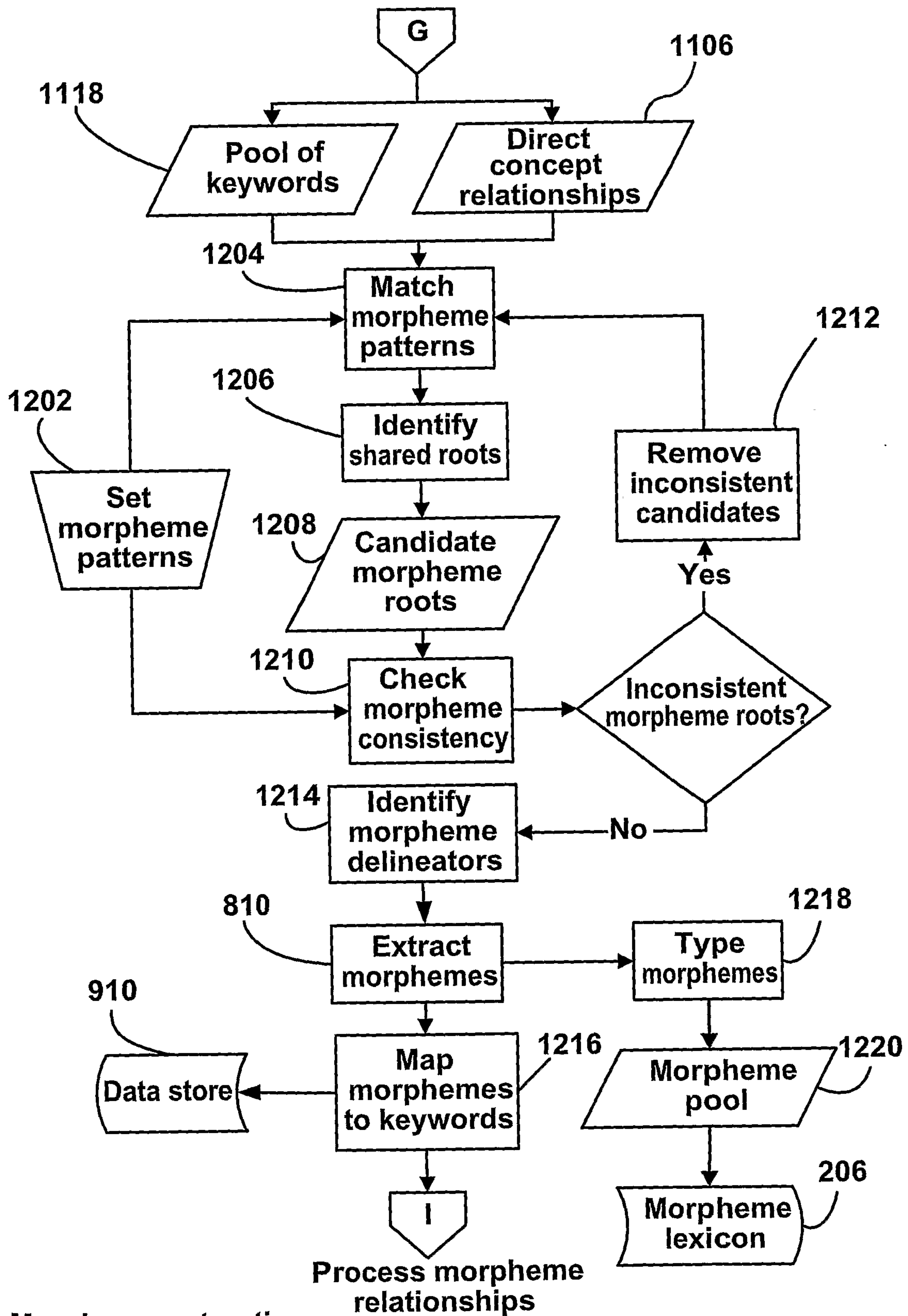
Morpheme extraction Figure 8
