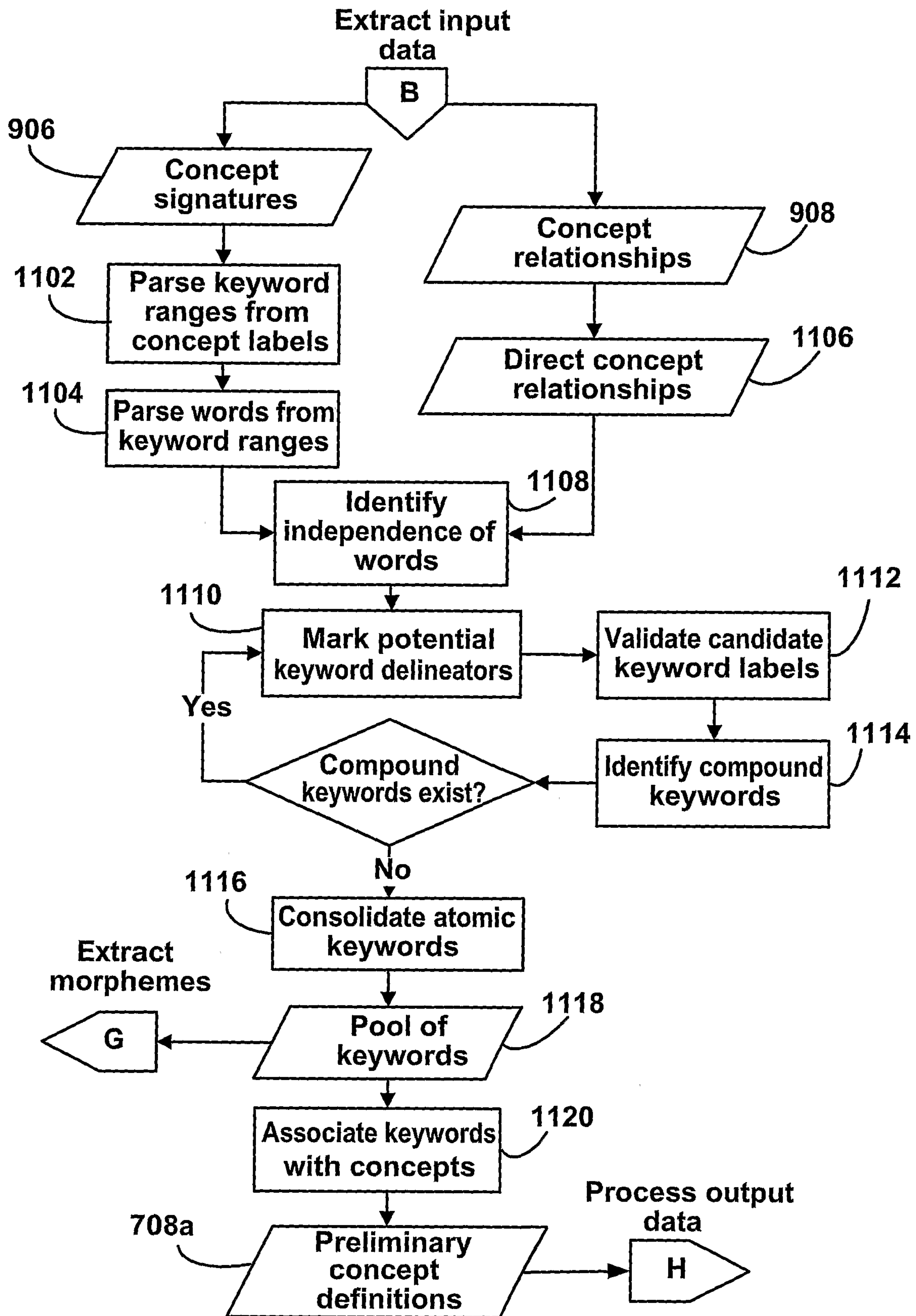
Extracting preliminary concept definitions Figure 7
