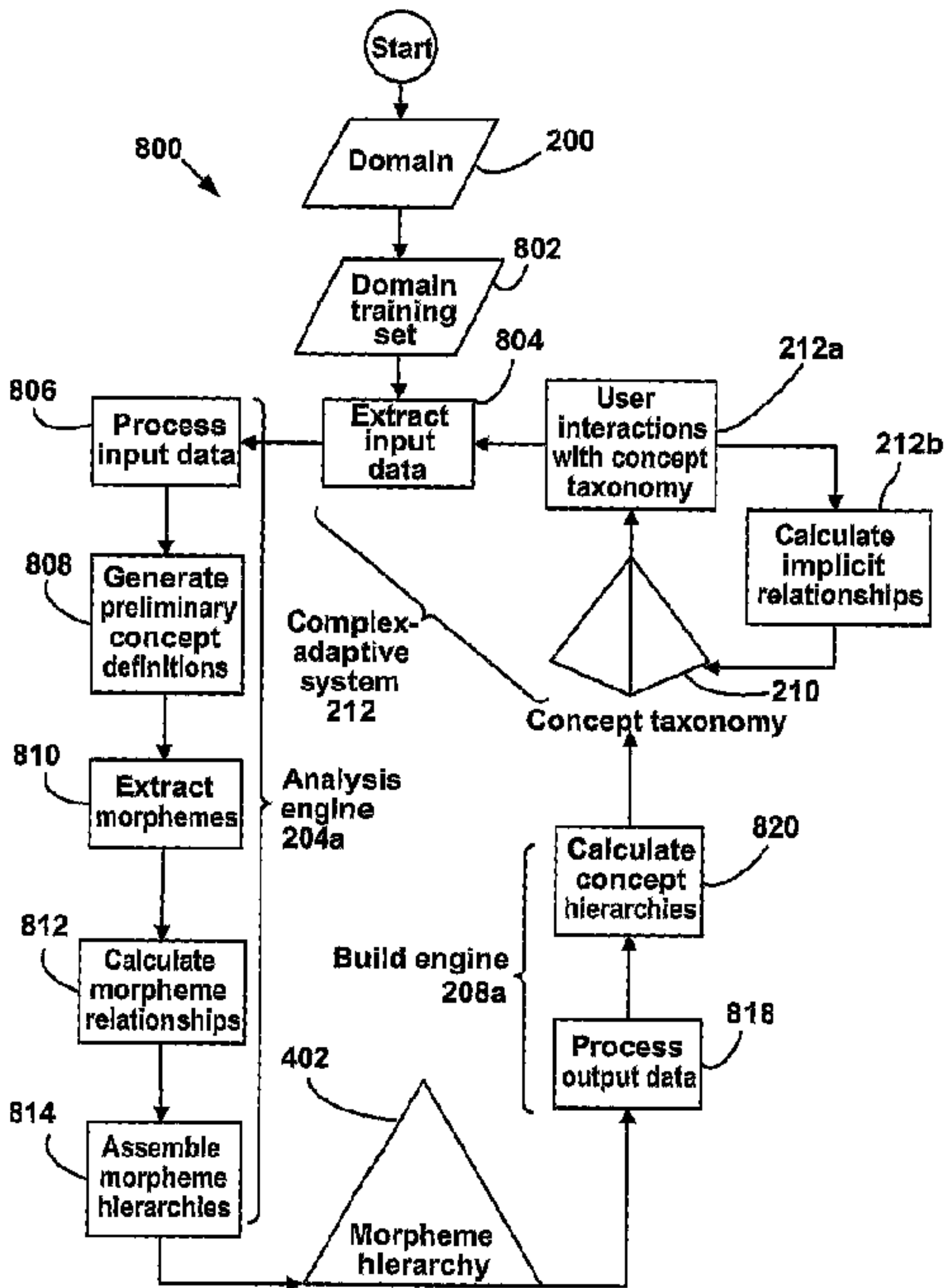
Overview of system methods
