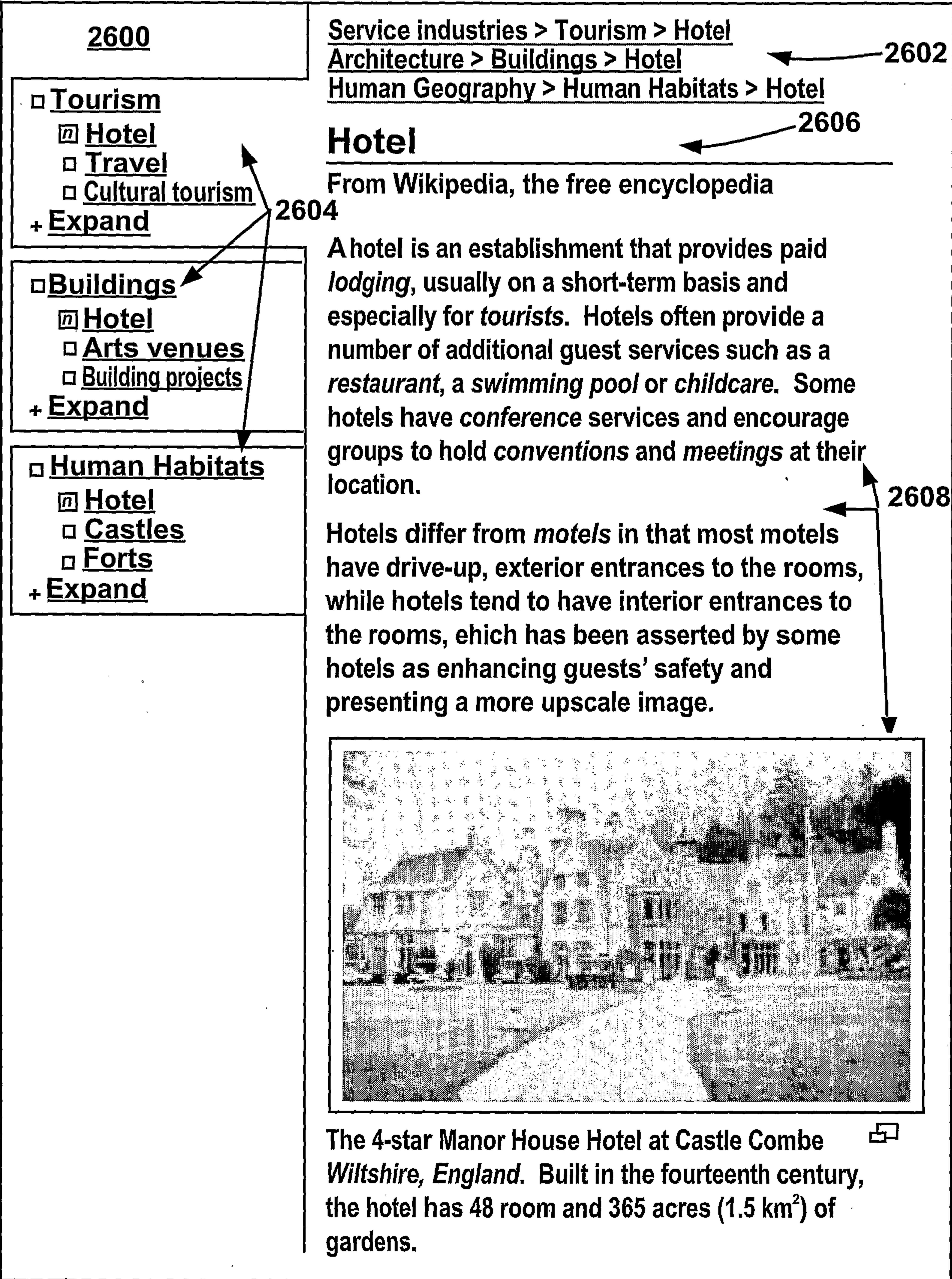
Presentation of concept taxonomy views Figure 34
