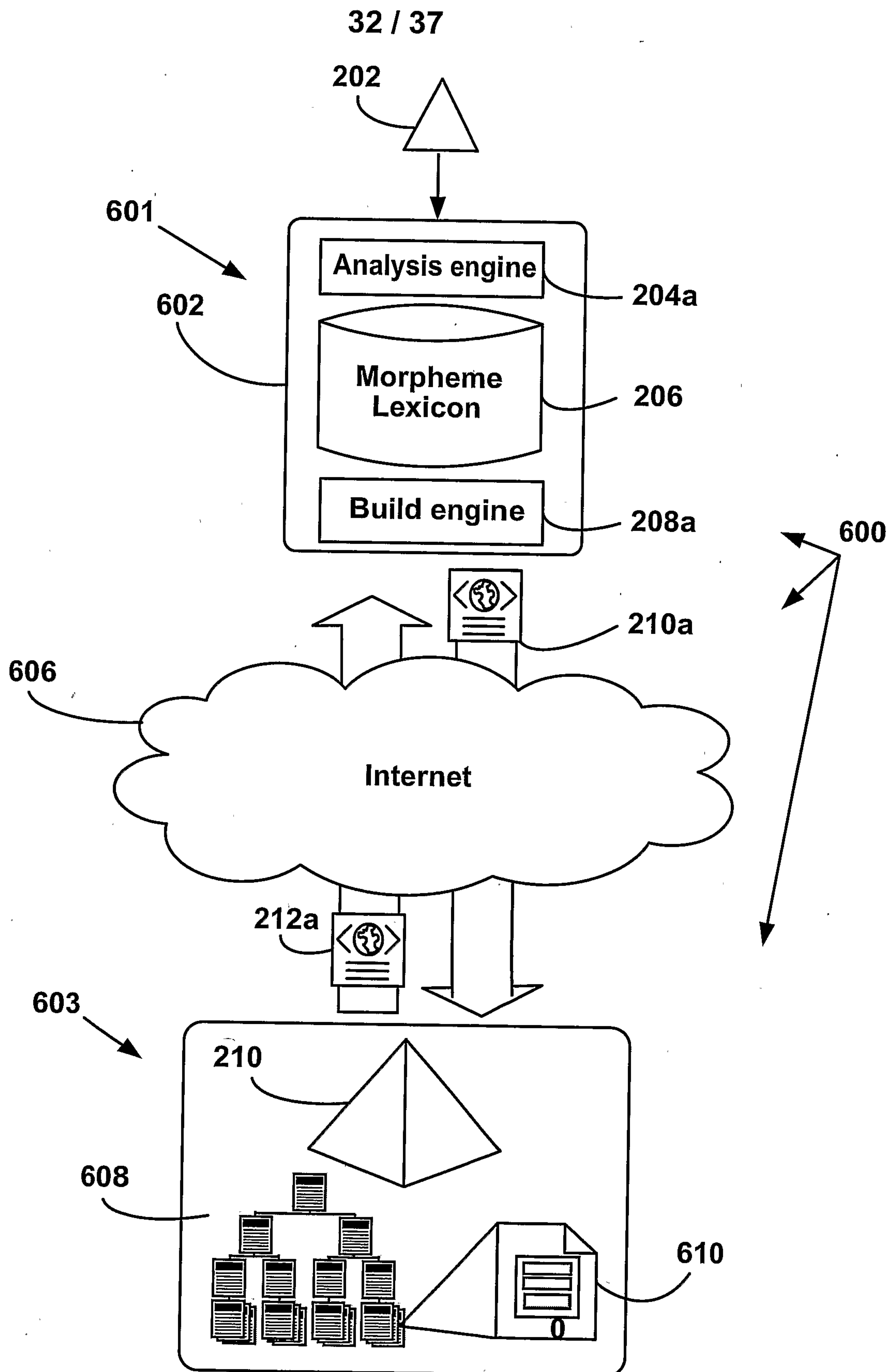
System overview Figure 32
