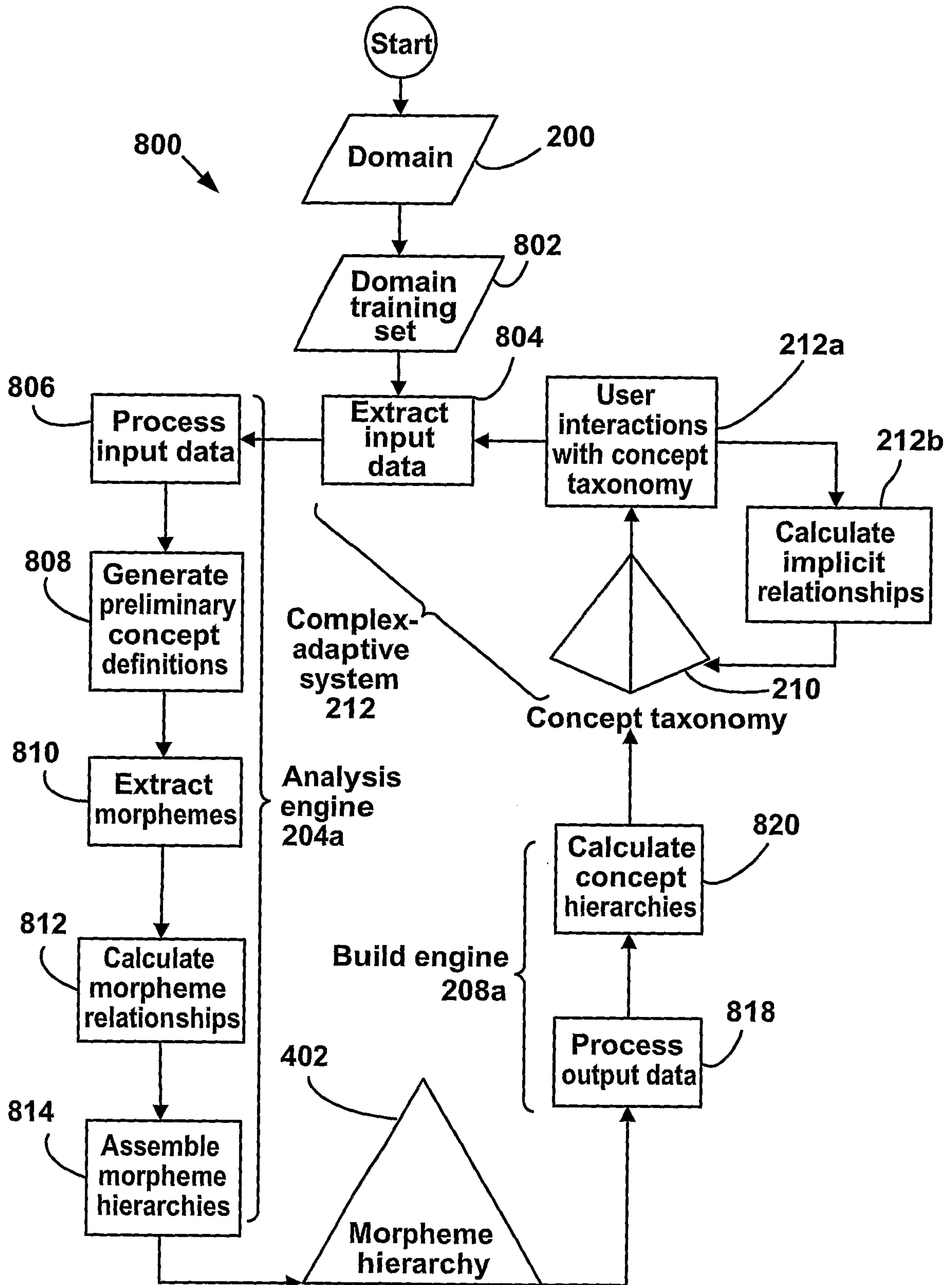
Overview of system methods Figure 4
