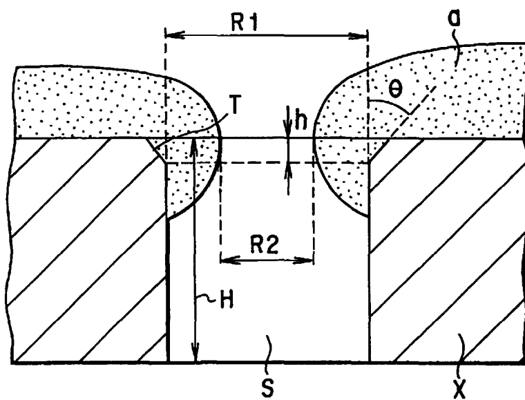
FIG. 6 (PRIOR ART)
