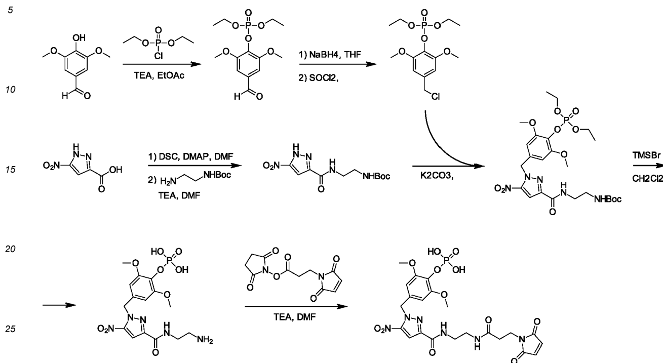
Scheme 1A: Synthesis of a Caged NP Hapten started with a substituted 4-hydroxybenzaldehyde.
