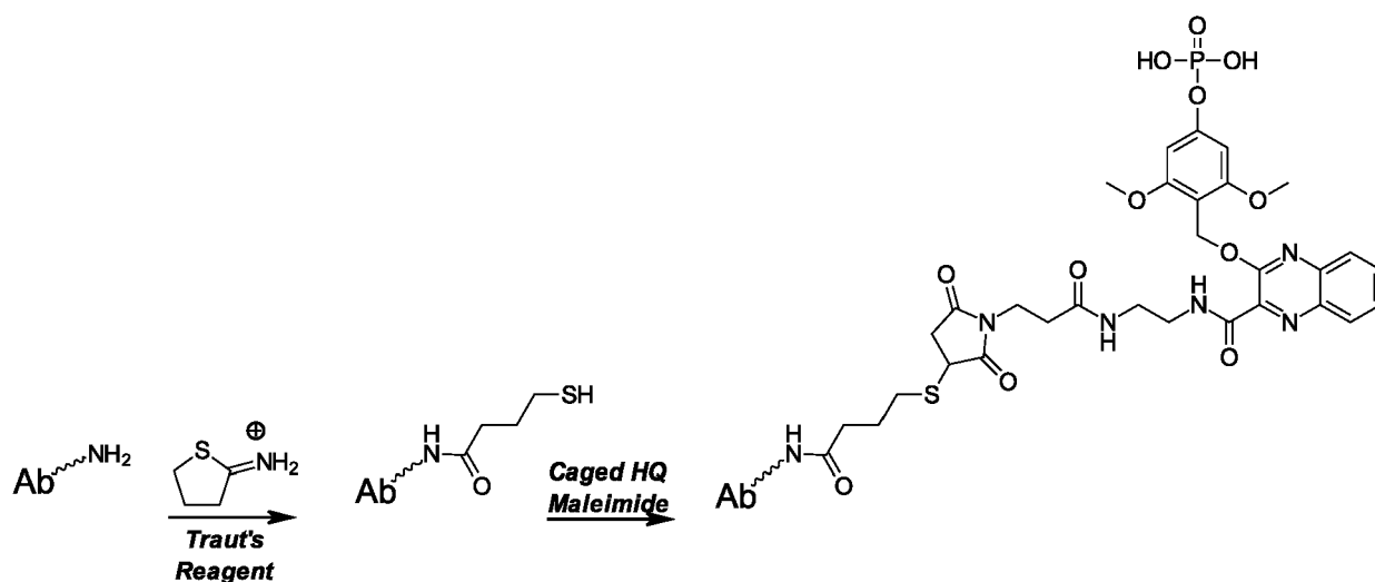
Scheme 2: Synthetic methodology illustrating the reaction between an amino group on an antibody ("Ab") with Traut's Reagent, followed by coupling of the resulting intermediate with a Caged HQ Maleimide.
