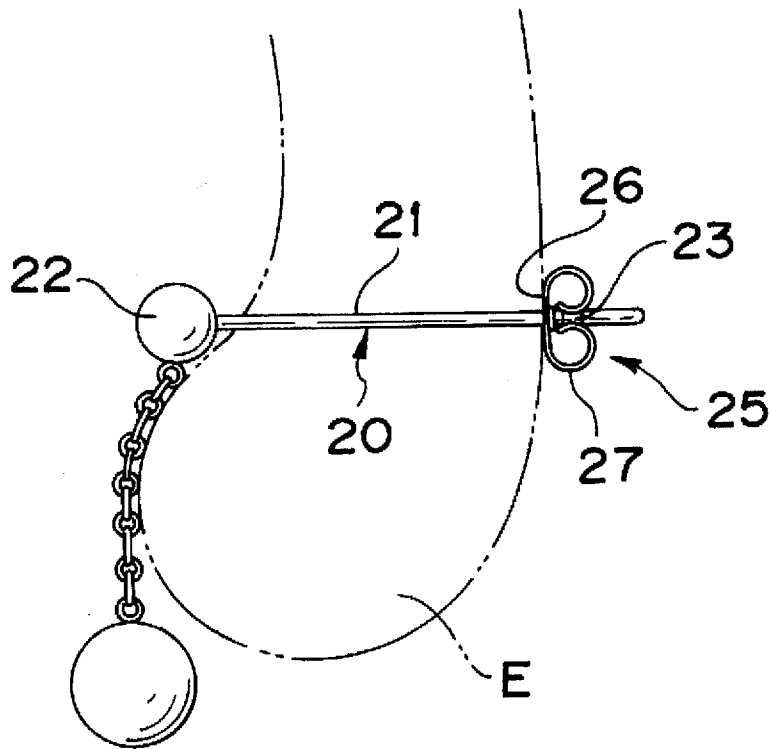
FIG. 8 PRIOR ART
