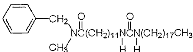
Structural Formula (1)
