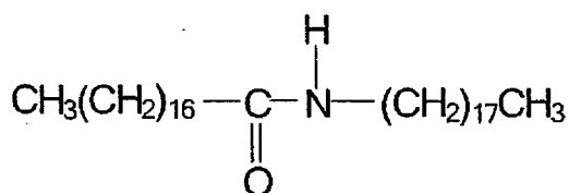
Structural Formula (3)
