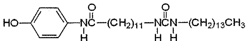
Structural Formula (1)
