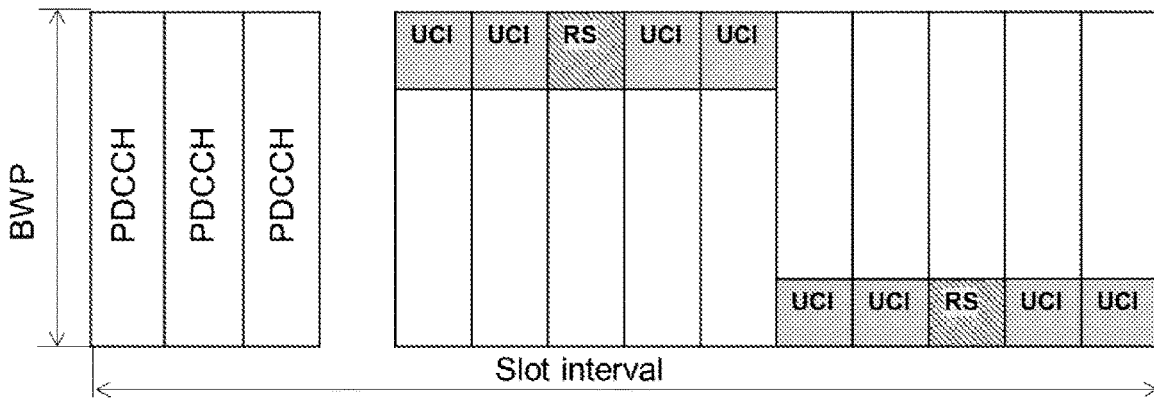
Long PUCCH with 10 symbols
