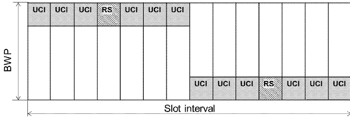
Long PUCCH with 14 symbols
