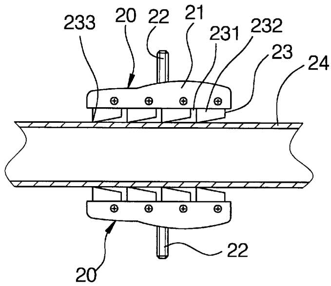
FIG. 5 PRIOR ART
