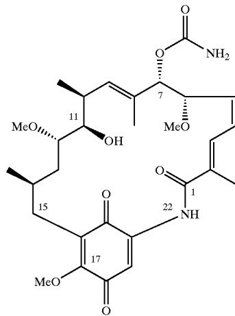
Geldanamycin
