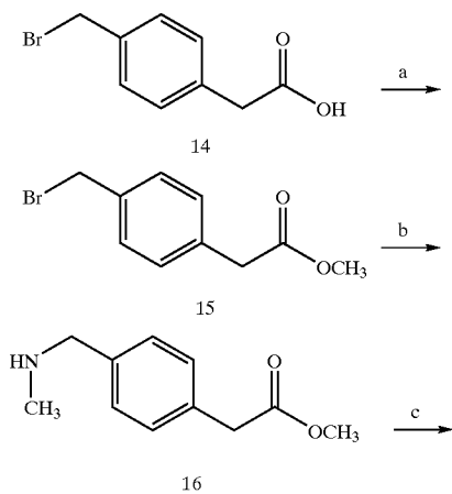
Scheme 3:
