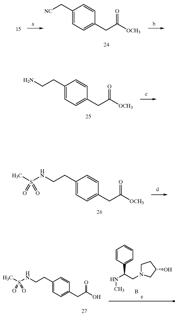
Scheme 5:
