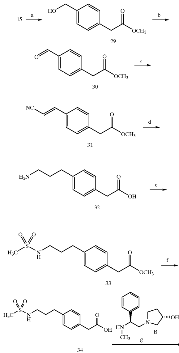
Scheme 6:
