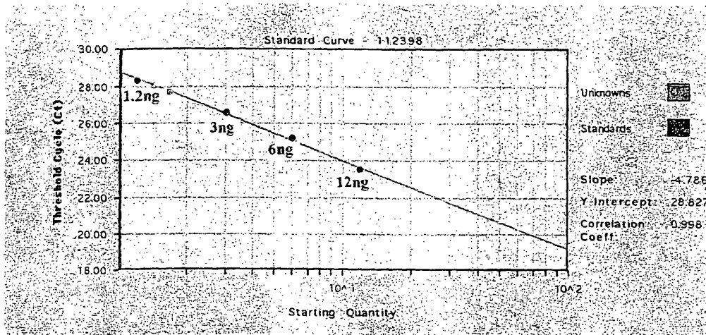
Figure 1. Standard Curve for DNA as Evaluated by TaqMan Amplification with the \beta -actin Gene after 40 PCR cycles
