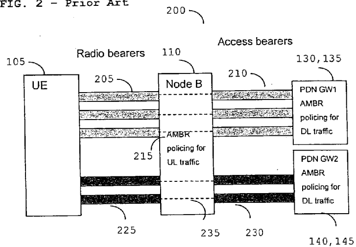
FIG. 2 - Prior Art
