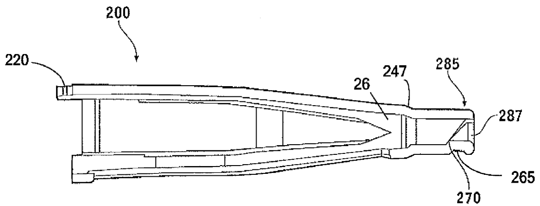
FIG. 24 SECTION C-C
