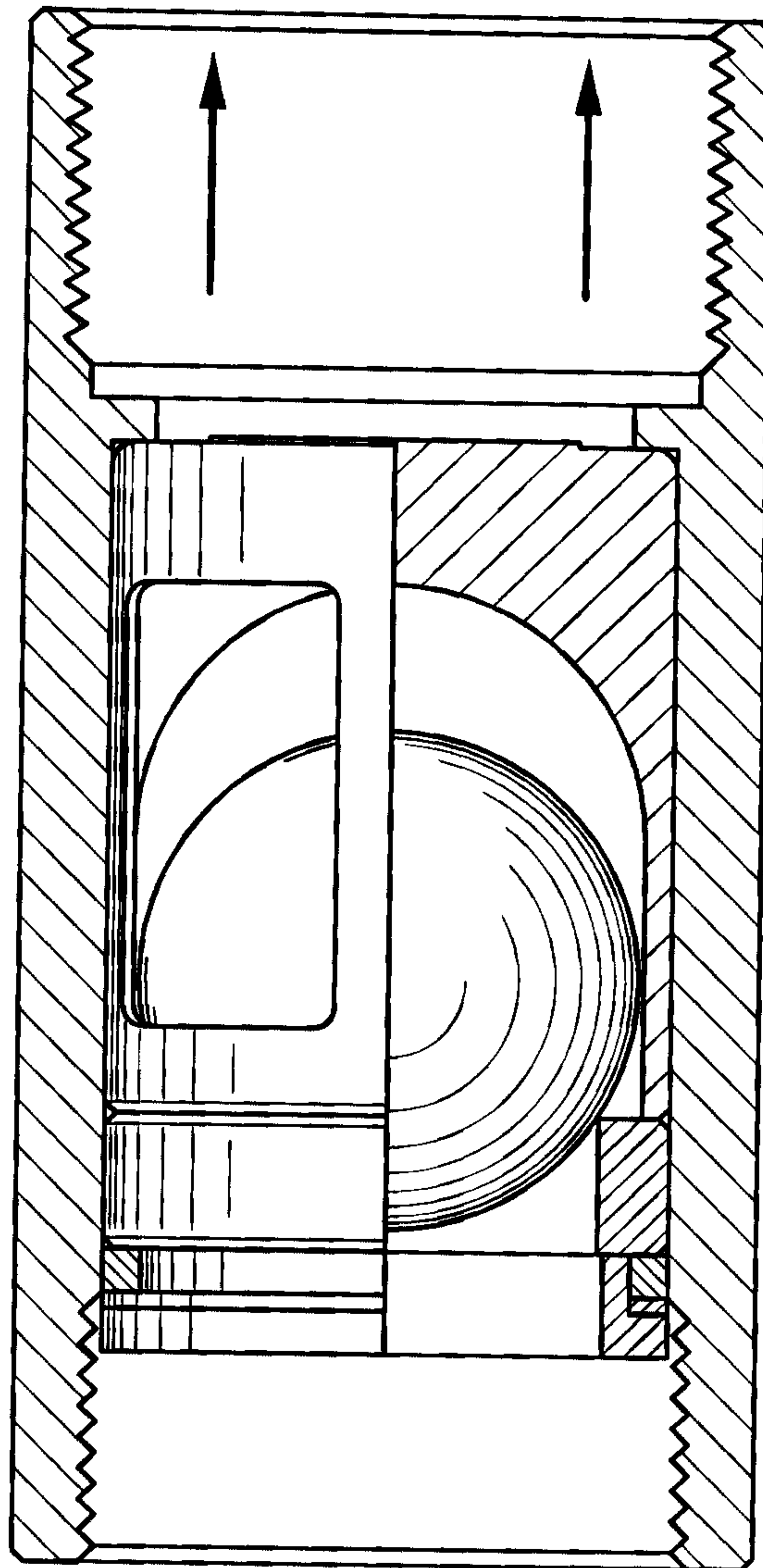
FIG. 1 (Prior Art)
