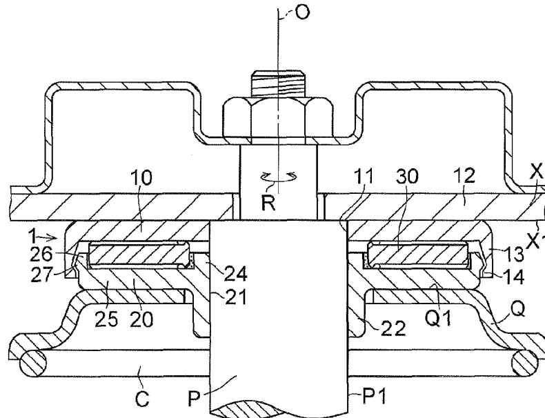
FIG. 15 (PRIOR ART)
