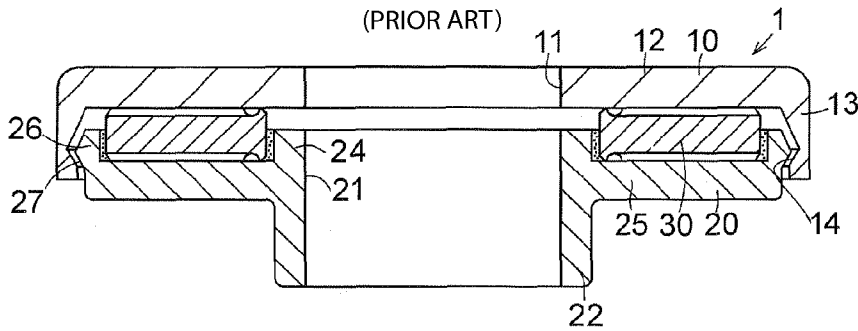
FIG. 15 (PRIOR ART)
