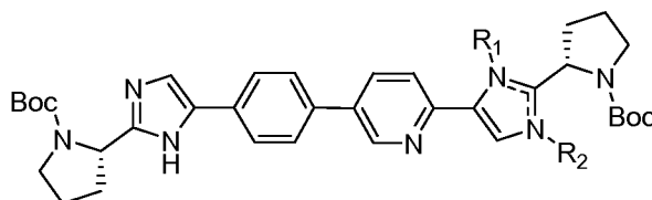
146f: ( R_1 = H, R_2 = SEM ) or ( R_1 = SEM, R_2 = H )
