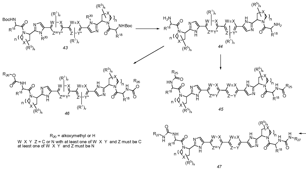
Scheme 10: Starting Material 29
