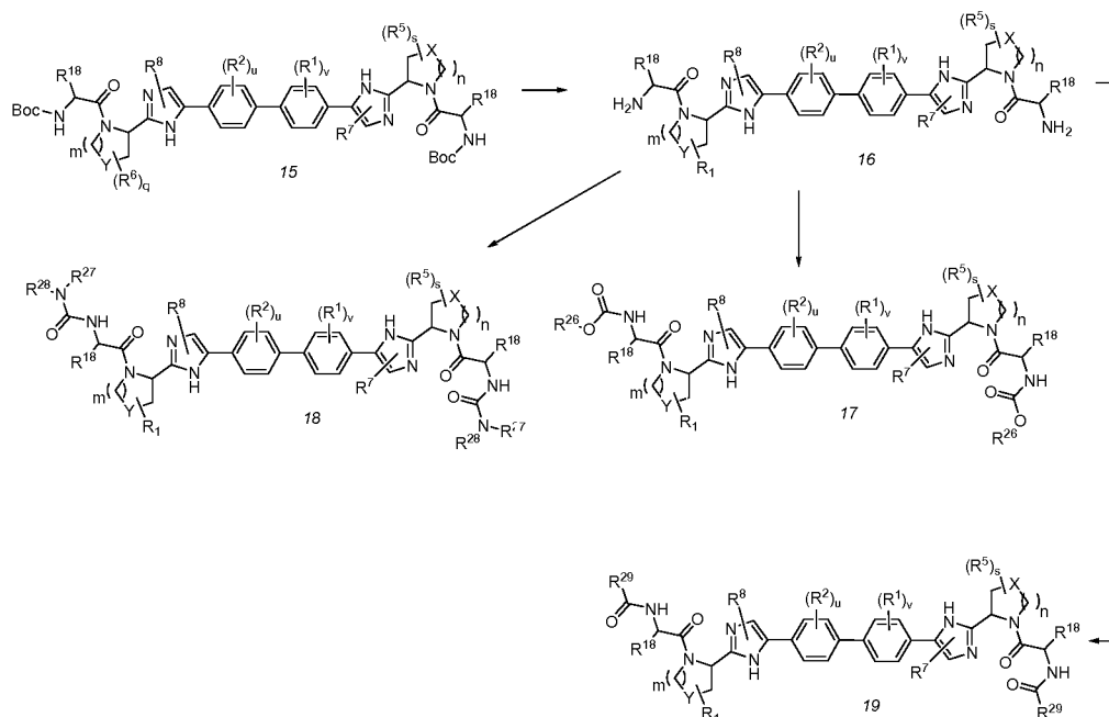
Scheme 4: Symmetric Biphenyls
