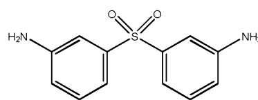
3,3'-DDS
