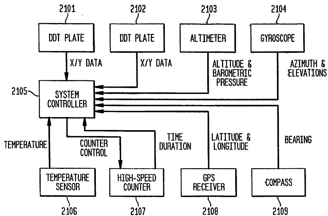
RSTL INPUT COMPONENT BLOCK DIAGRAM
