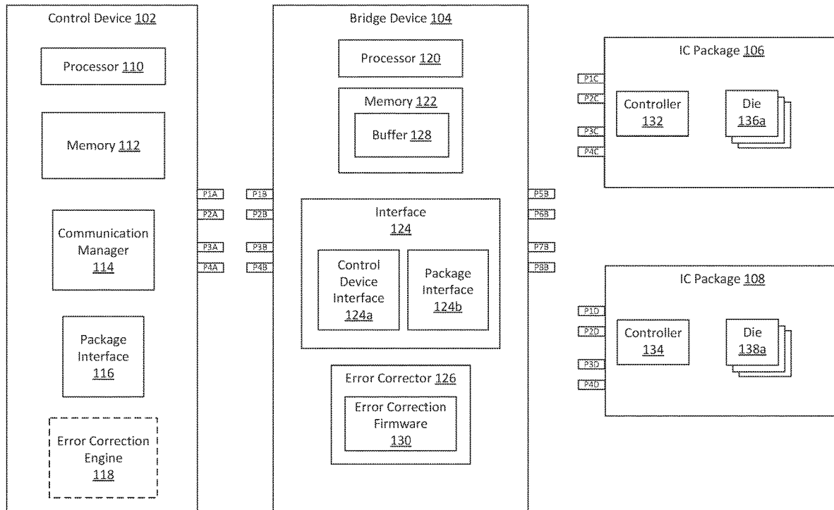
Communication System 100
