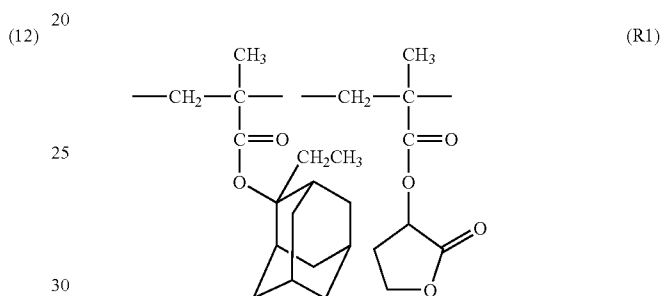
Synthesis Example 16
