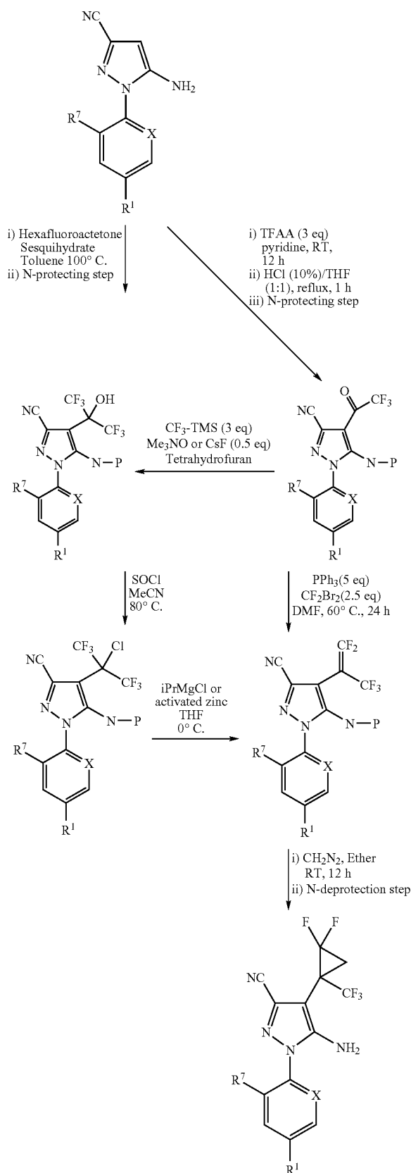
Scheme 3
