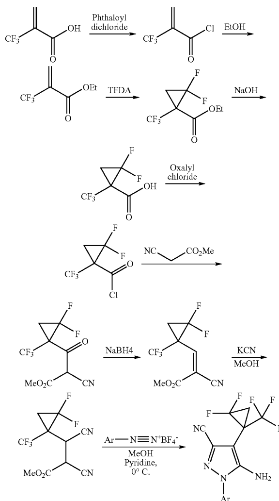
Scheme 2
