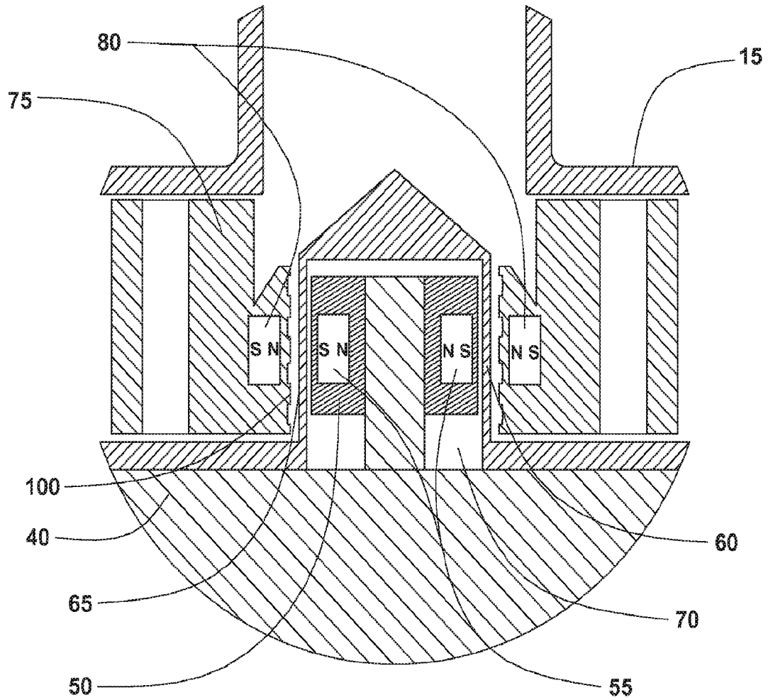
FIG 4 (DETAIL C)
