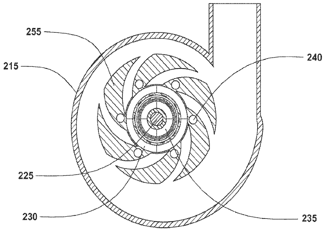
FIG. 19 (Section G-G)
