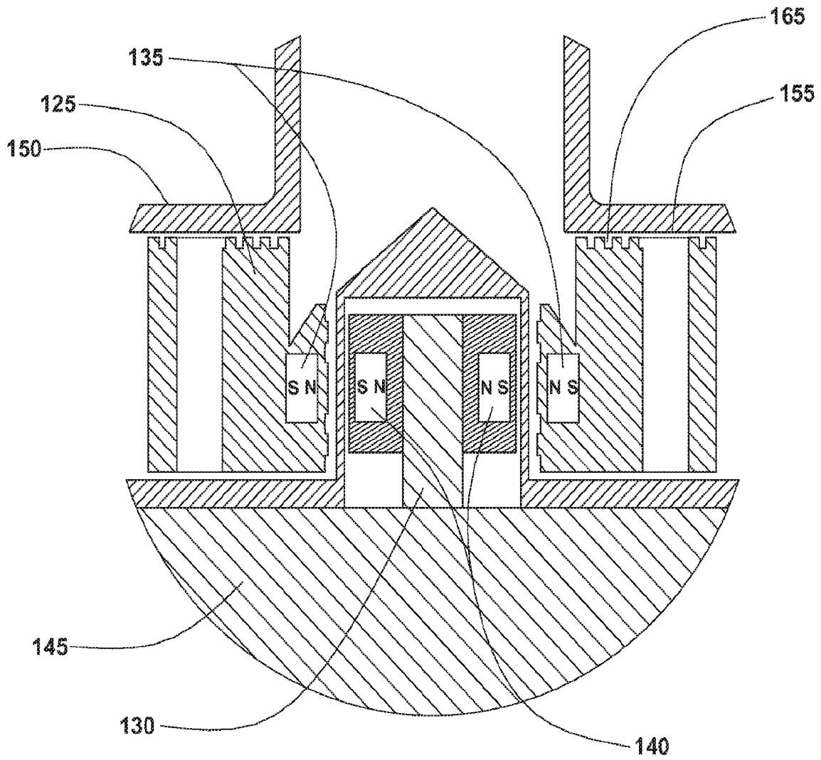
FIG. 13 (DETAIL D)
