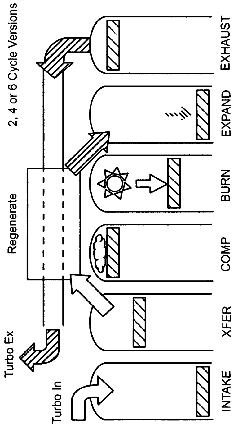
Extremely High Efficiency 4-Cycle, 7-Phase Engine
